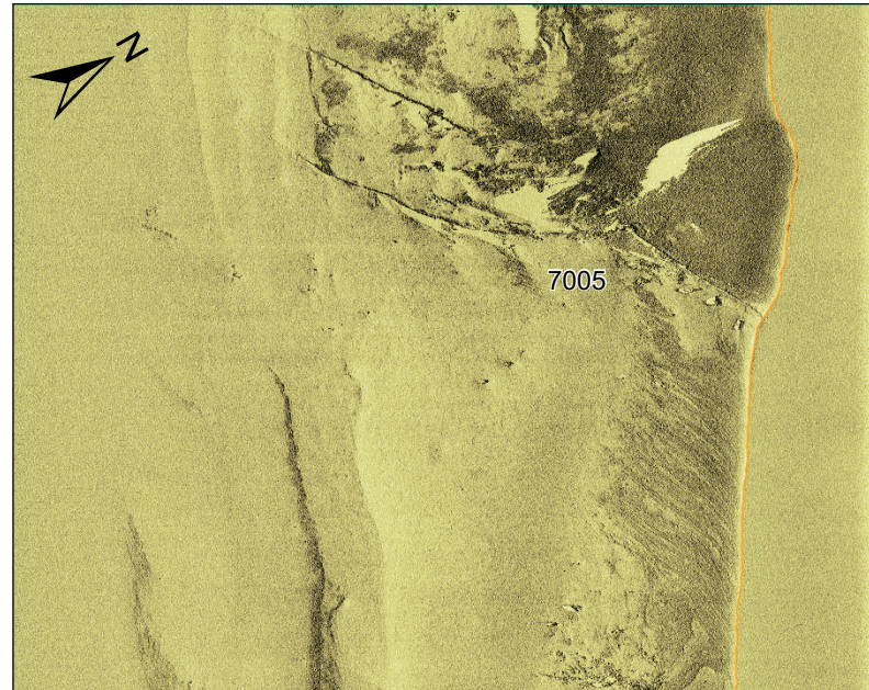
Sidescan sonar waterfall image showing debris field 7005, measuring 8.6 x 7.8 x 0.6 m
