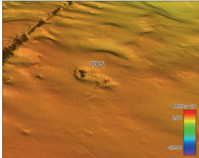
Gridded multibeam echosounder image showing debris field 7005, measuring 8.6 x 7.8 x 0.6 m, looking north, x 1 vertical exaggeration
