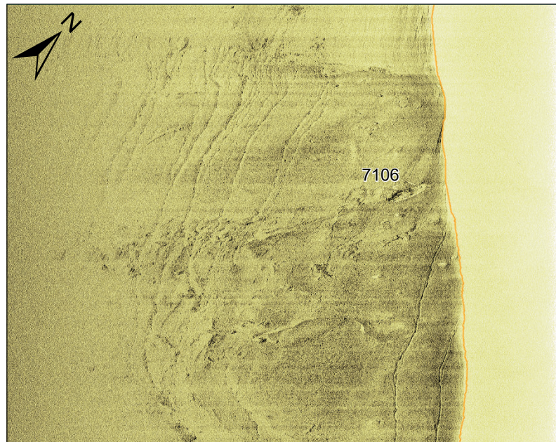
Sidescan sonar waterfall image showing debris field 7106, measuring 12.1 x 11.4 x 0.3 m
