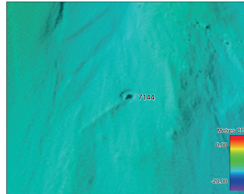
Gridded multibeam echosounder image showing debris field 7144, measuring 8.7 x 1.4 x 0.2 m
