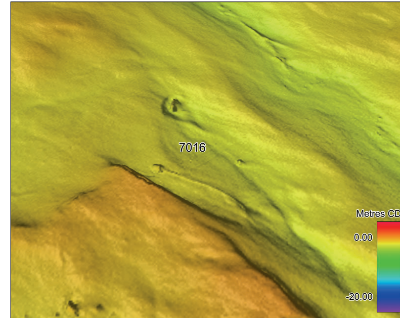
Gridded multibeam echosounder image showing debris field 7016, measuring 27.5 x 16.0 x 0.6 m, looking north, x 1 vertical exaggeration
