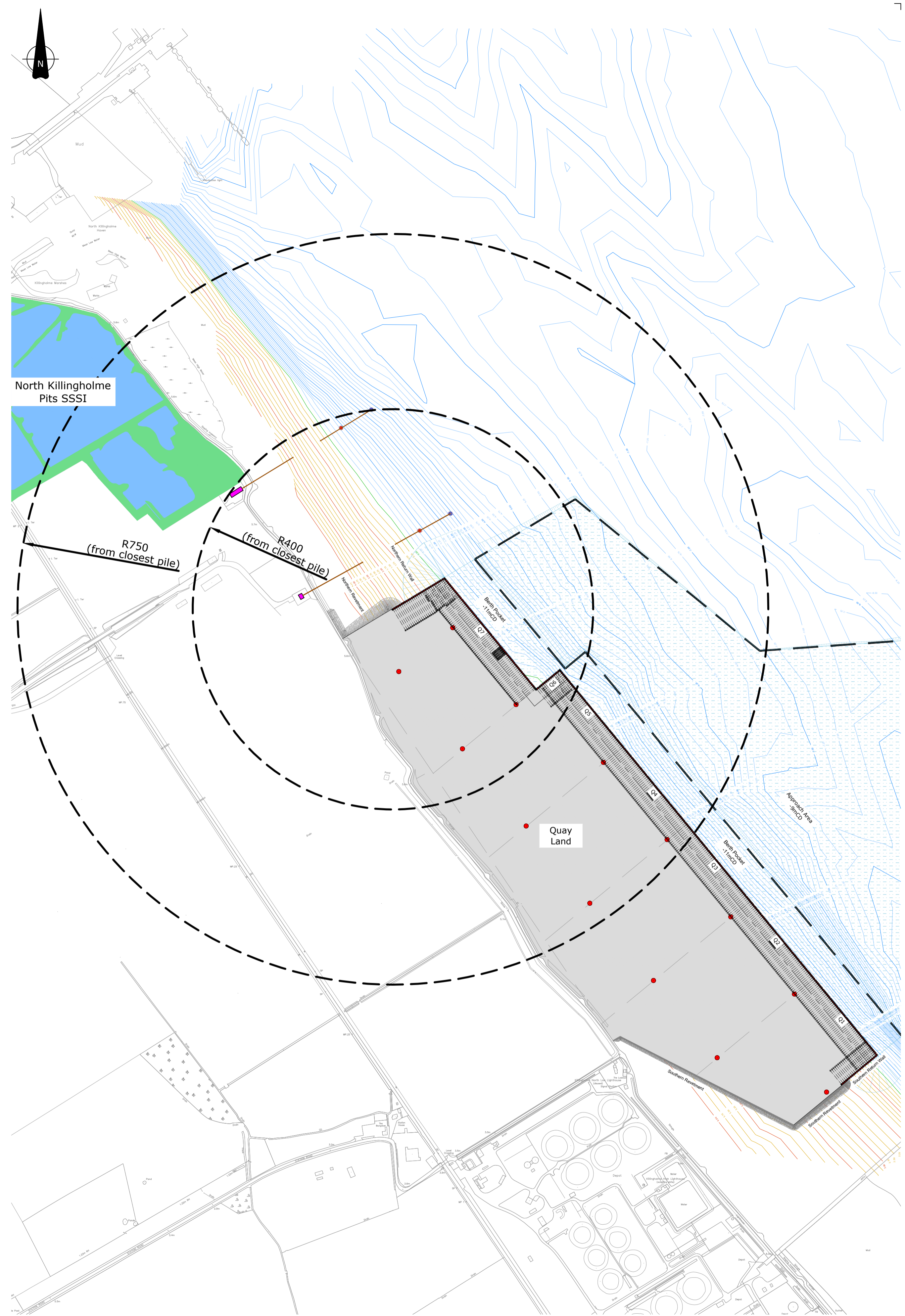
Proposed Quay Design Scale 1:5000
