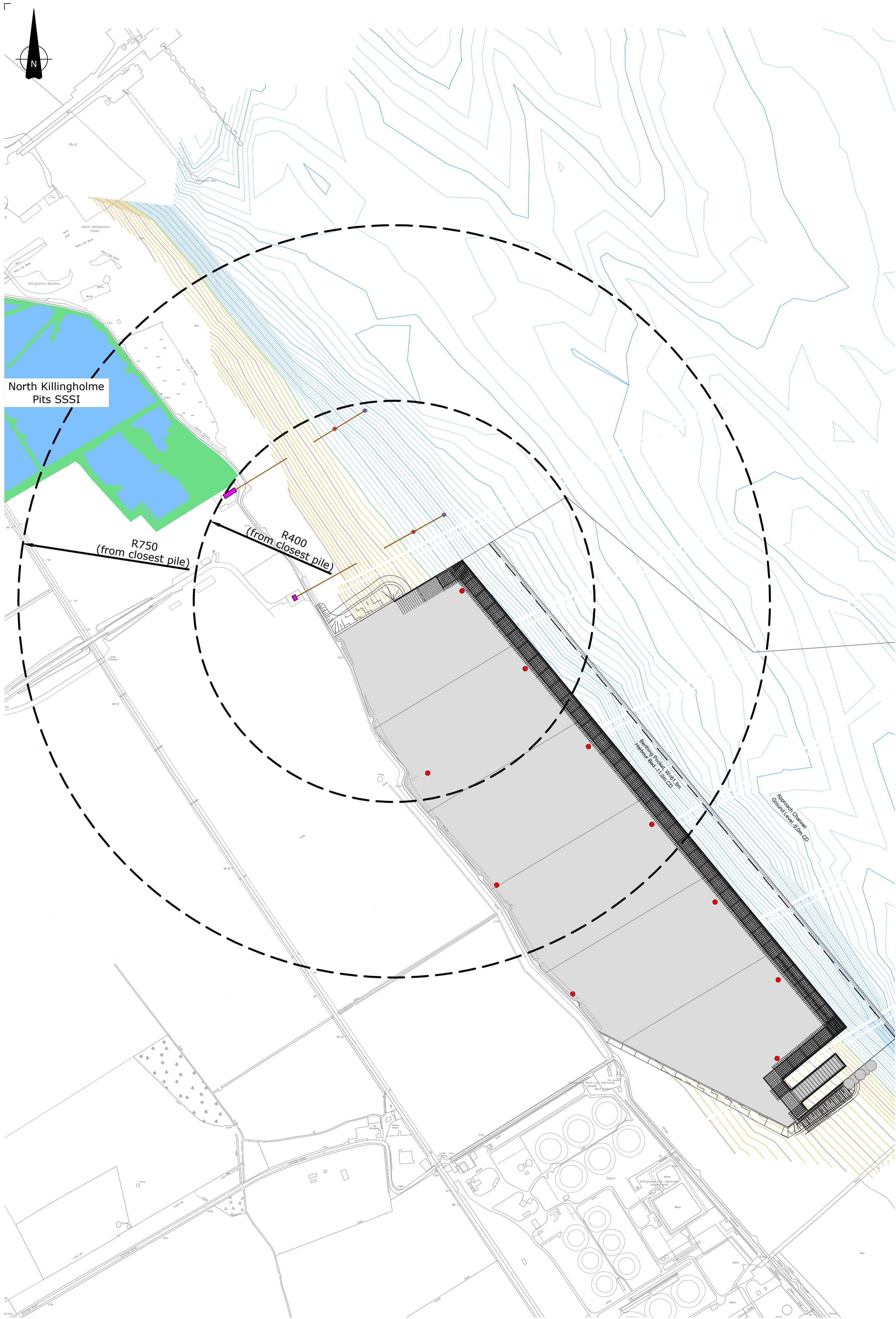
Consented Quay Design Scale 1:5000
