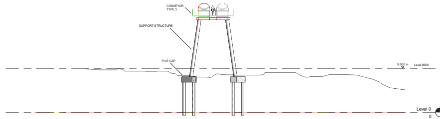
Section F-F 1:200
