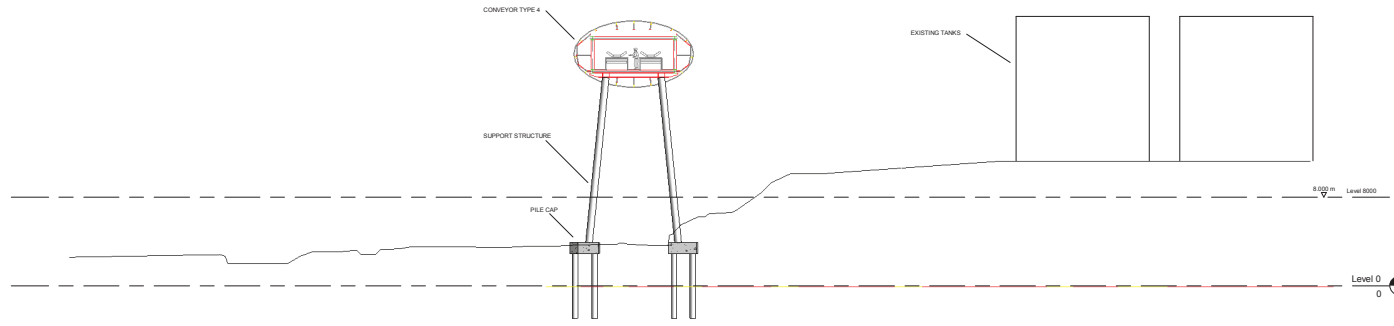
Section E-E 1:200
