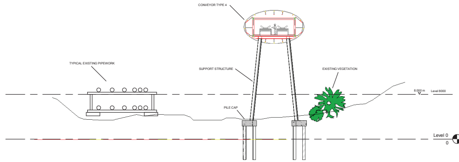
Section B-B 1:200
