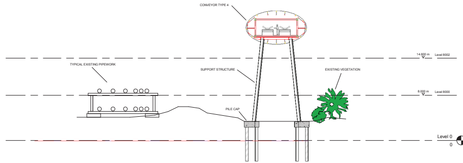
Section B-B 1:200
