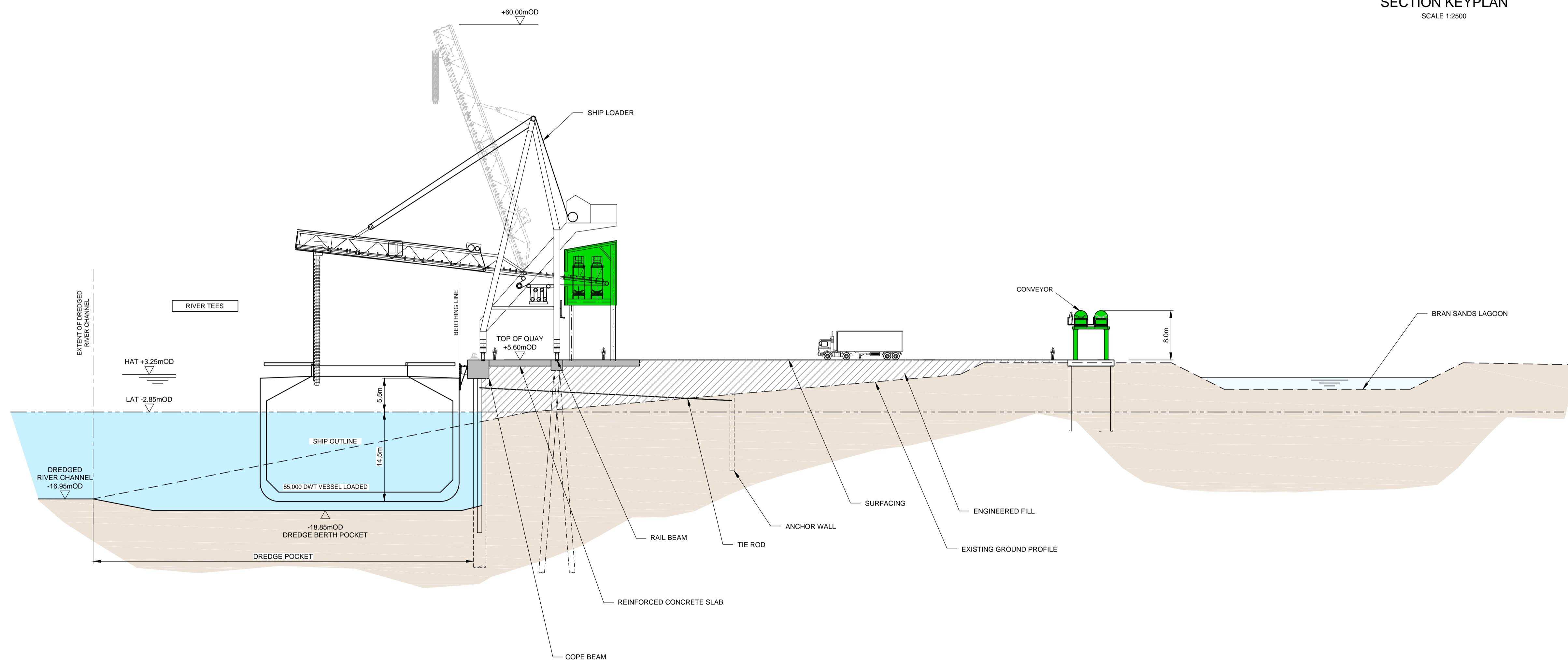
CROSS SECTION OF SOLID QUAY (SEE SK91)
