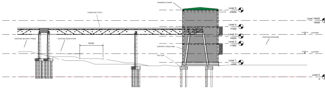
Section C-C 1:200
