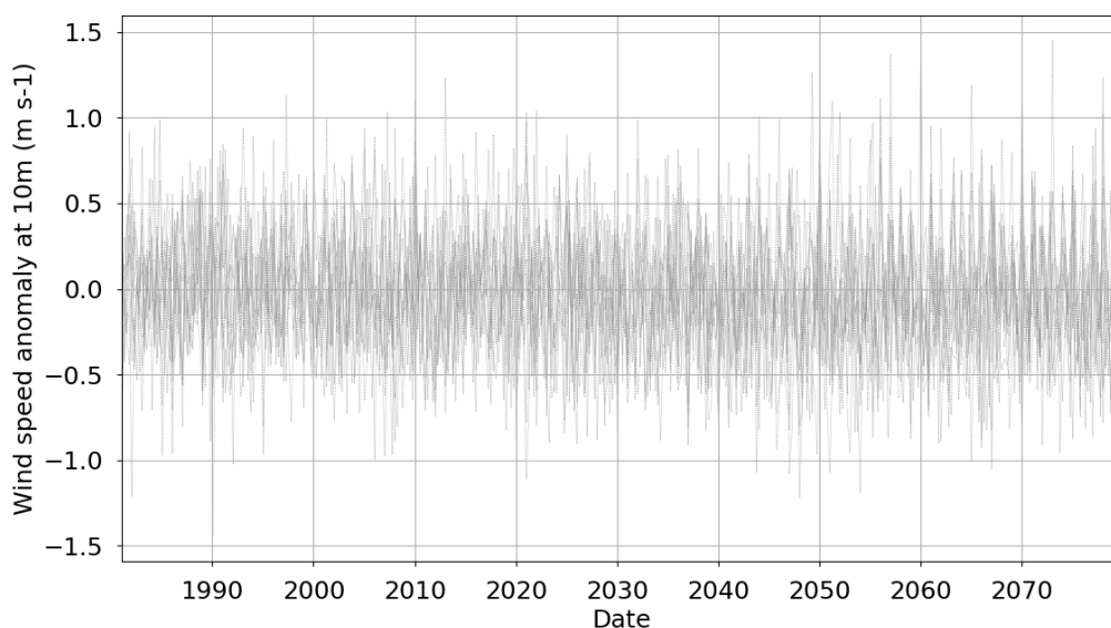
Figure 14-16 - Projected seasonal average wind speed anomaly (1980-2080)
