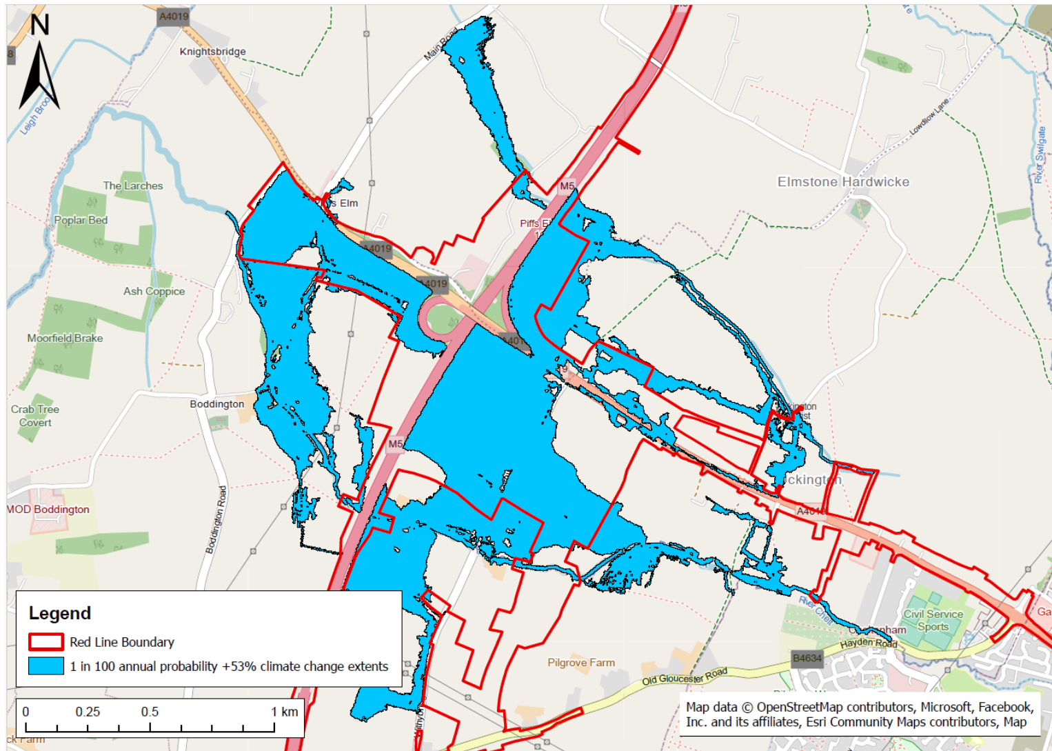
Figure B 10-5 - Extent of flooding in 1 in 100-year storm event, without Scheme in place
