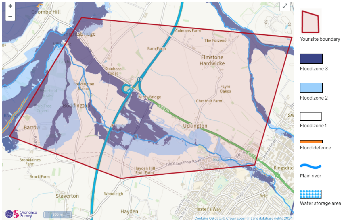
Figure B 10-2 - Environment Agency flood zones
