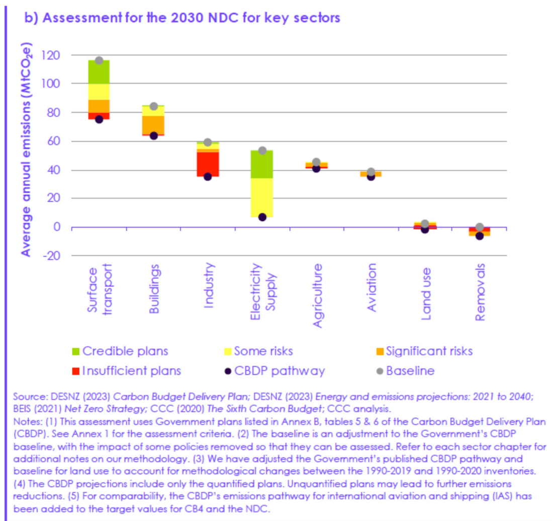
Figure 3: CCC Progress Report 2023, Fig 4b reproduced
