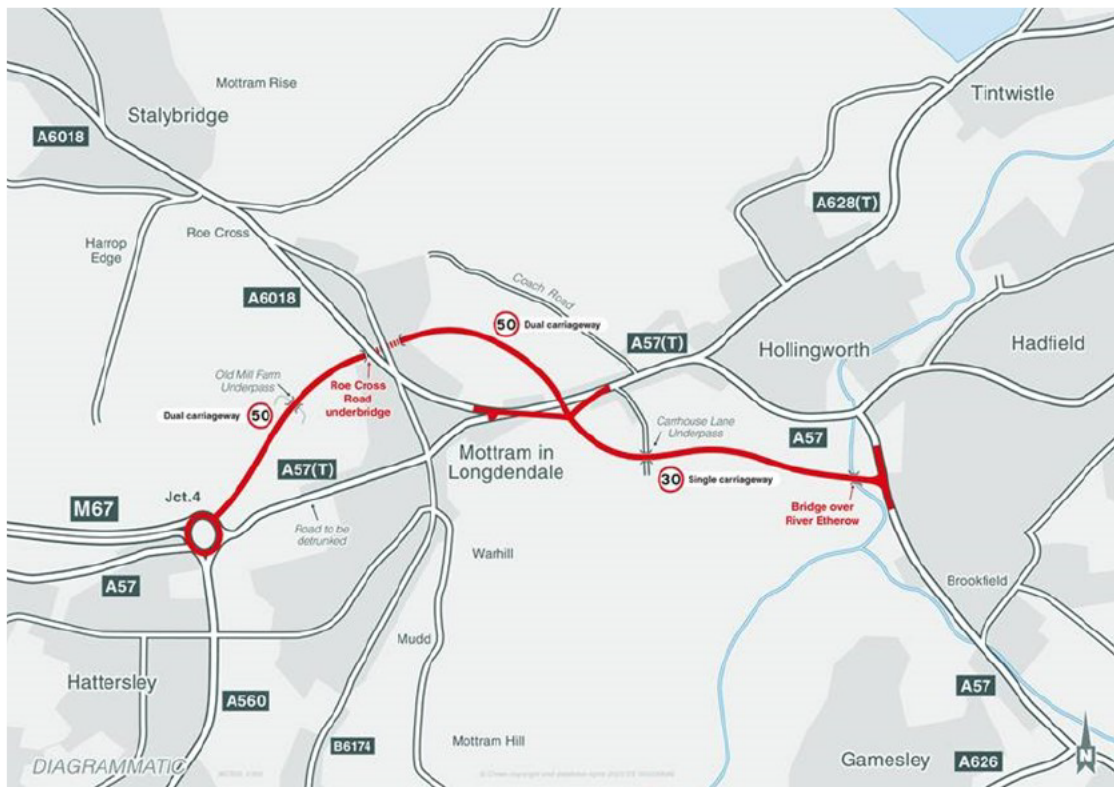
Insert 1 – Indicative Scheme Alignment
