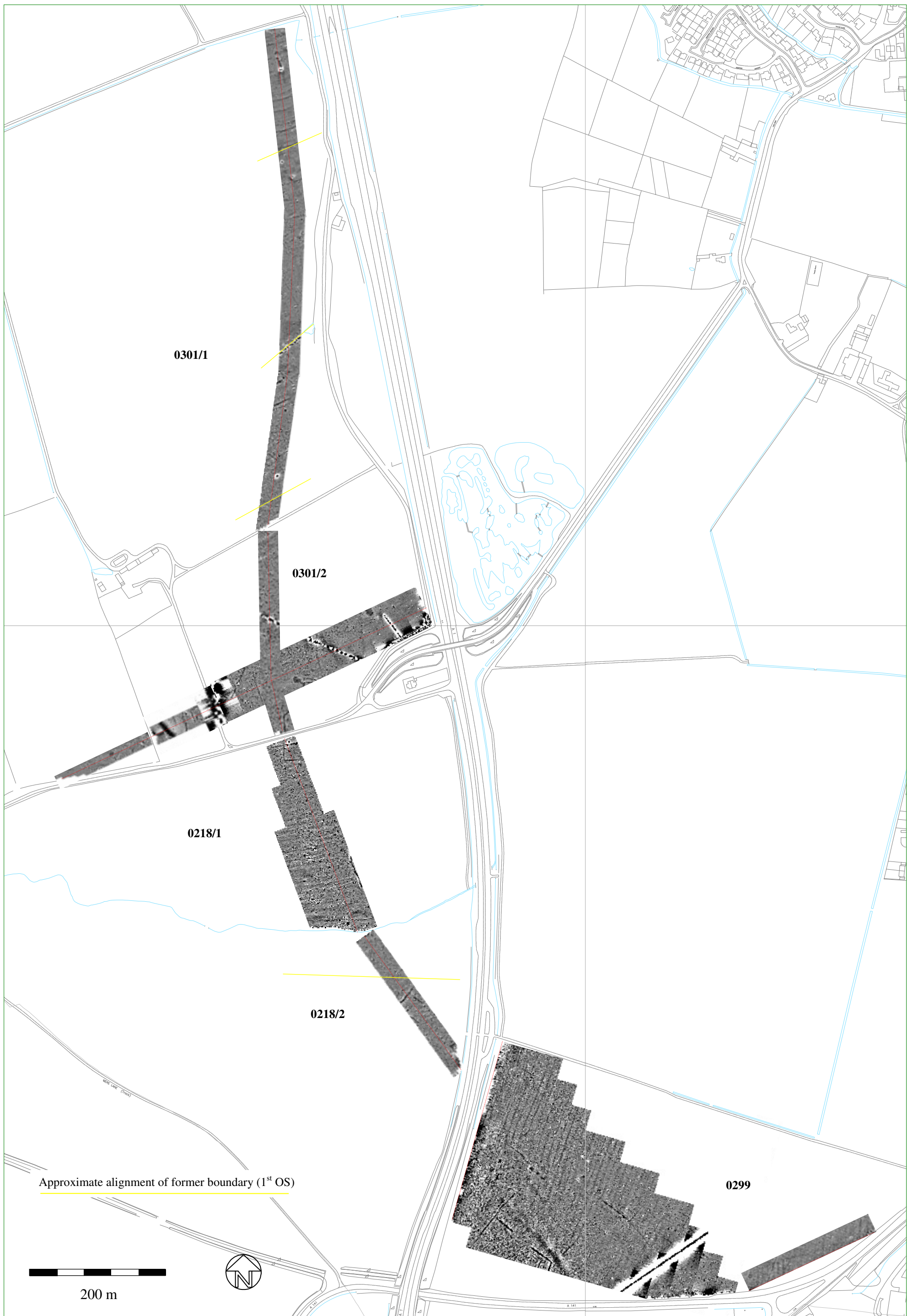
Fig 6: 0301/1 - 0299 1:5000
