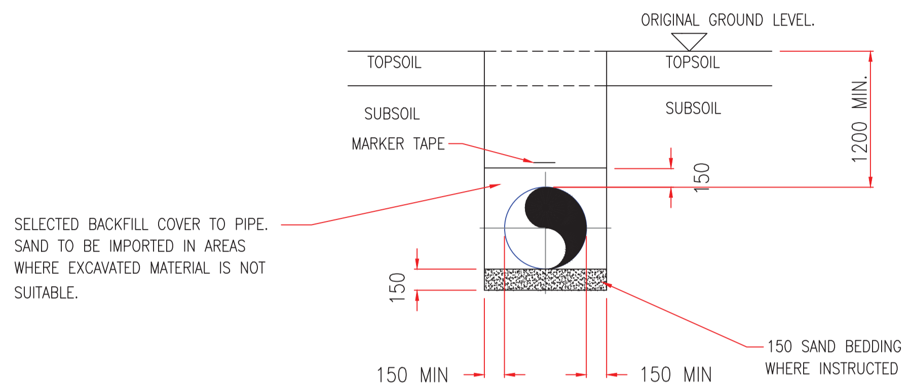
INSTALLATION OF PIPELINE WHERE BEDDING IS REQUIRED
