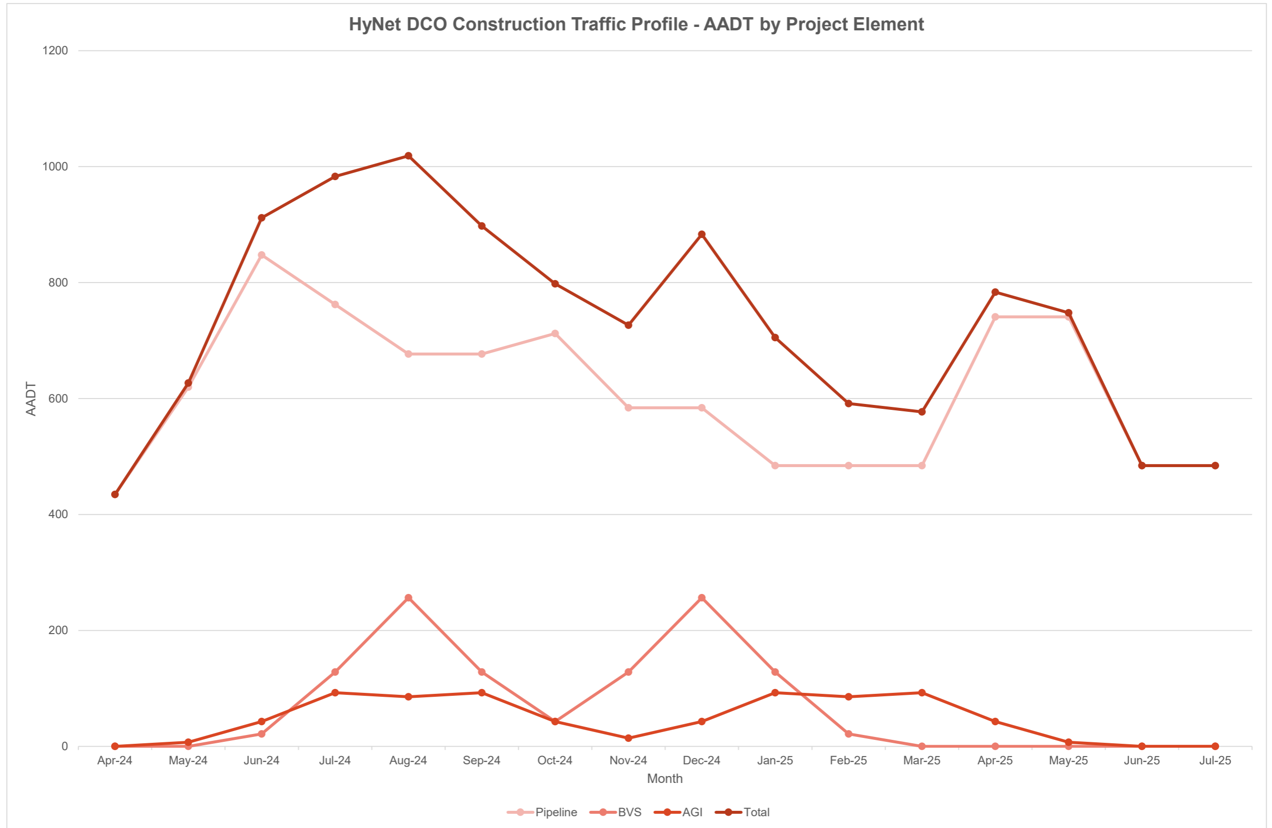
Insert 2: HyNet DCO Construction Traffic Profile - AADT by Project Element
