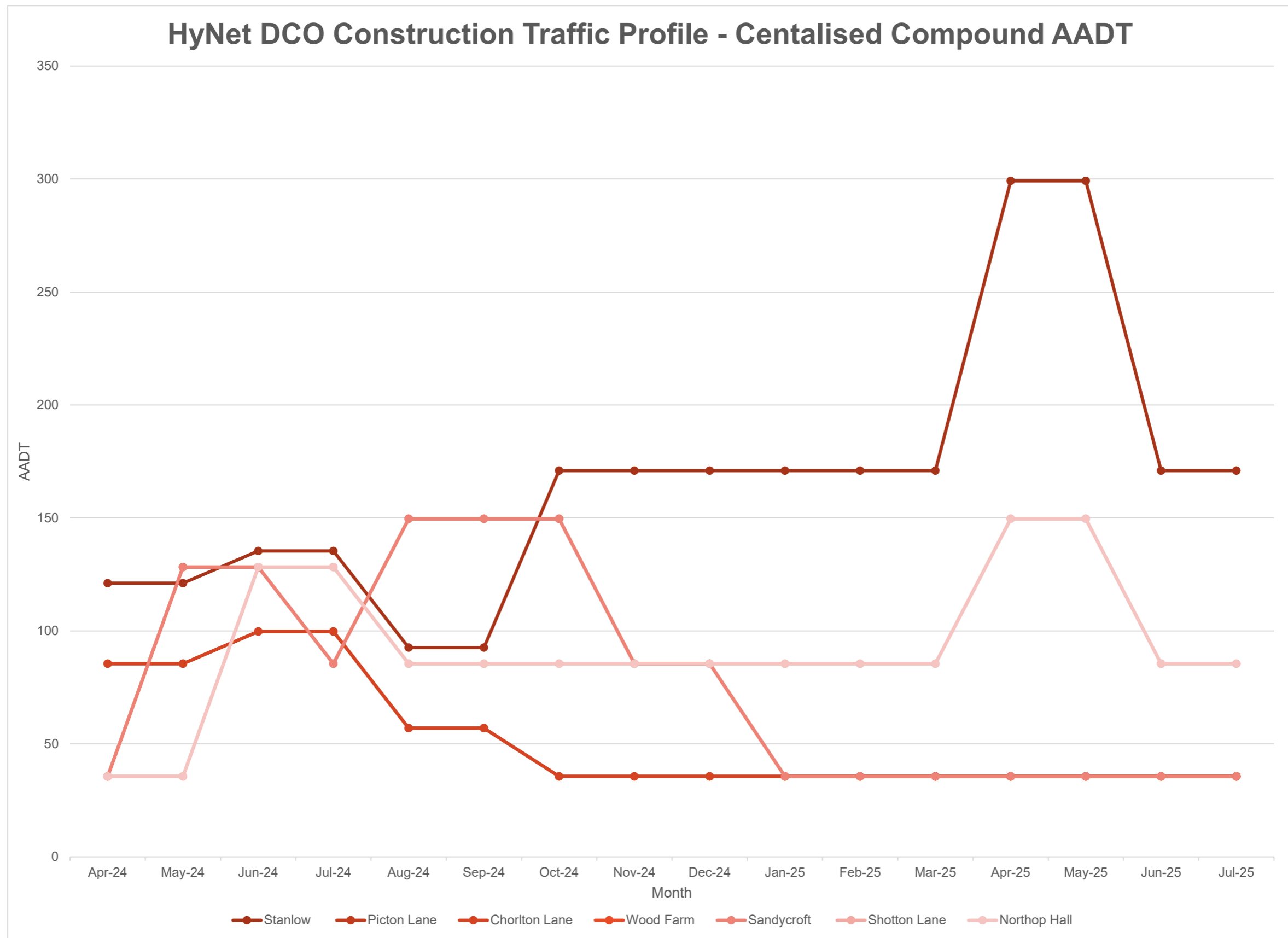
Insert 4: HyNet DCO Construction Traffic Profile - Centralised Compound AADT
