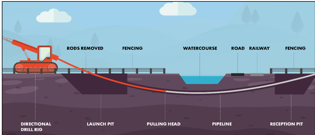
Image 2 – Illustration of a typical arrangement for trenchless crossing
