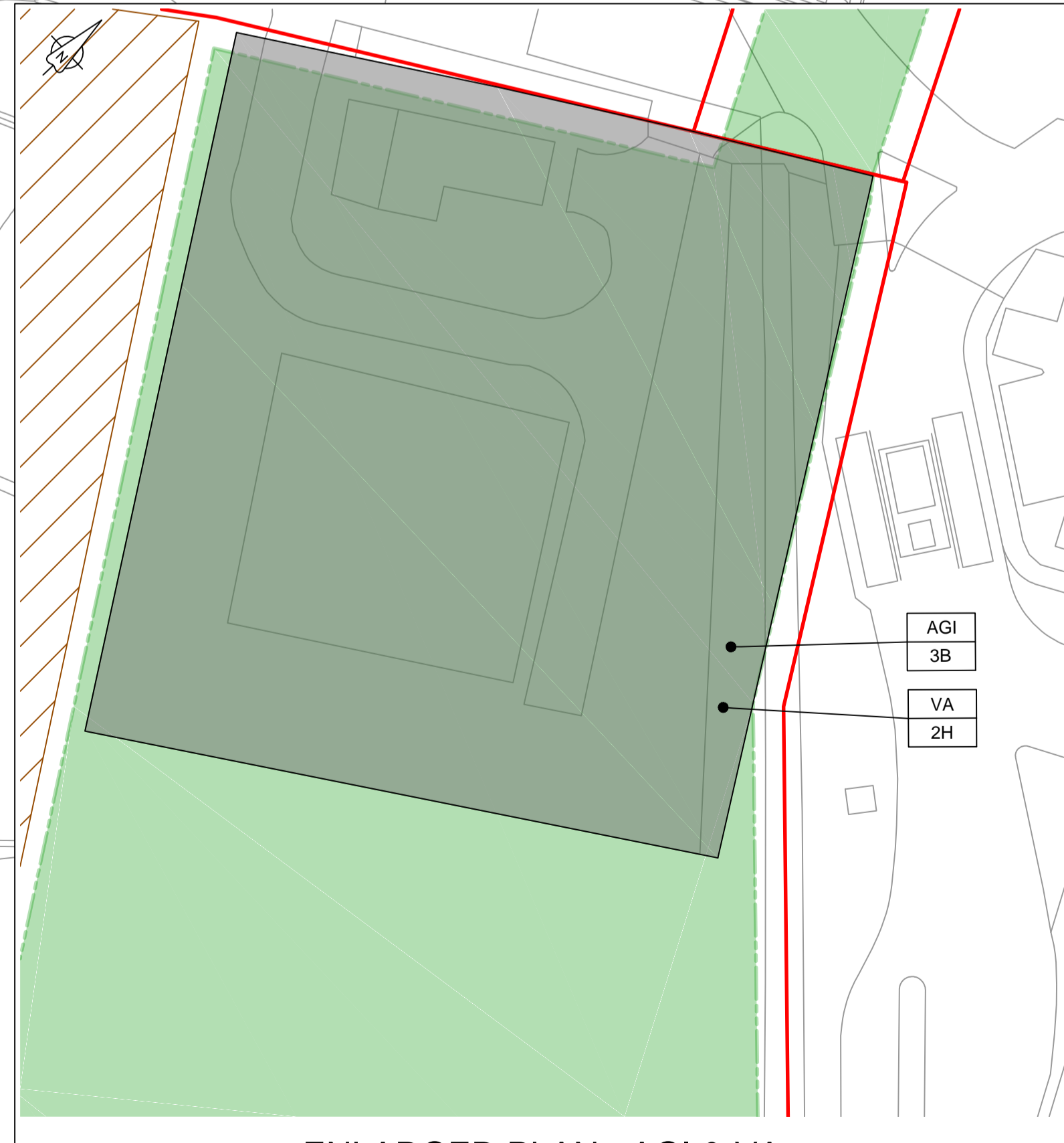
ENLARGED PLAN - AGI & VA SCALE 1:500
