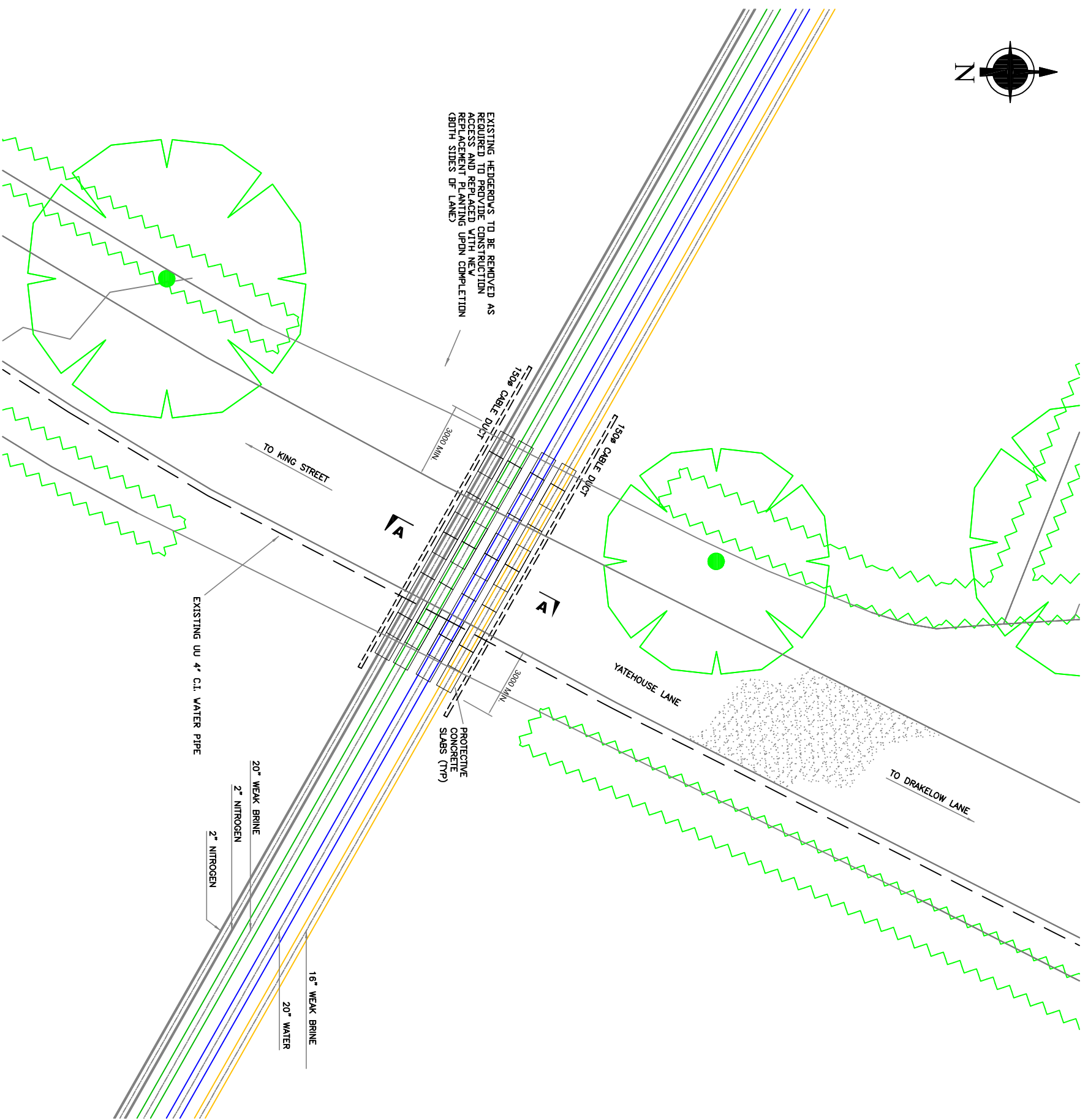
PLAN ON ROAD PIPELINE CROSSING YL2 1:200
