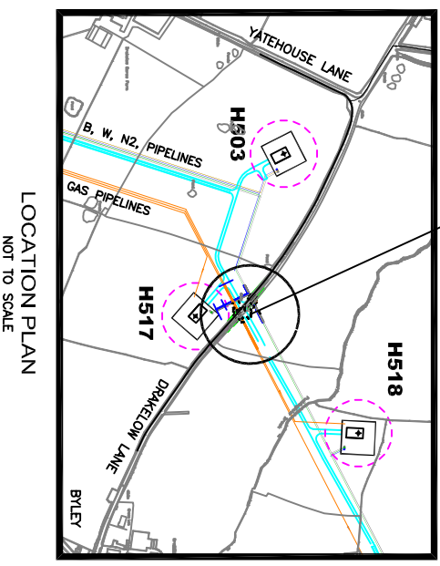
THIS DRAWING PIPELINE ROAD CROSSINGS DL3 AND DL4
