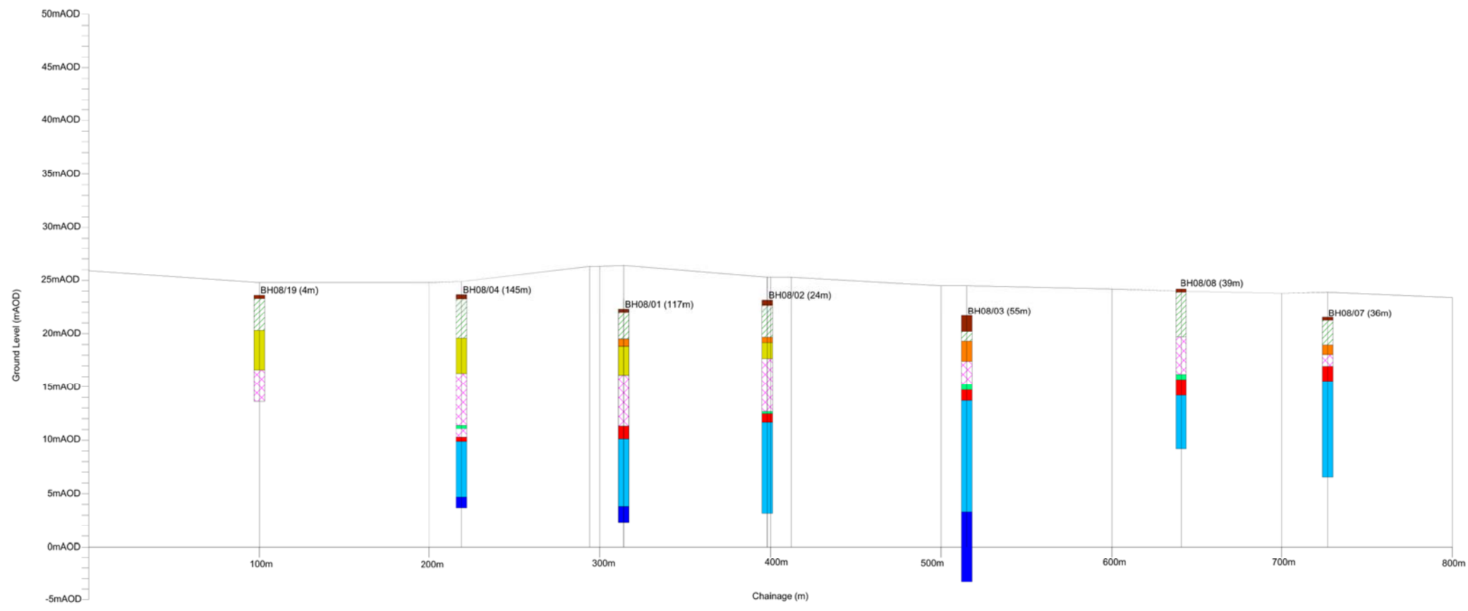
GEOLOGICAL SECTION 6-6
