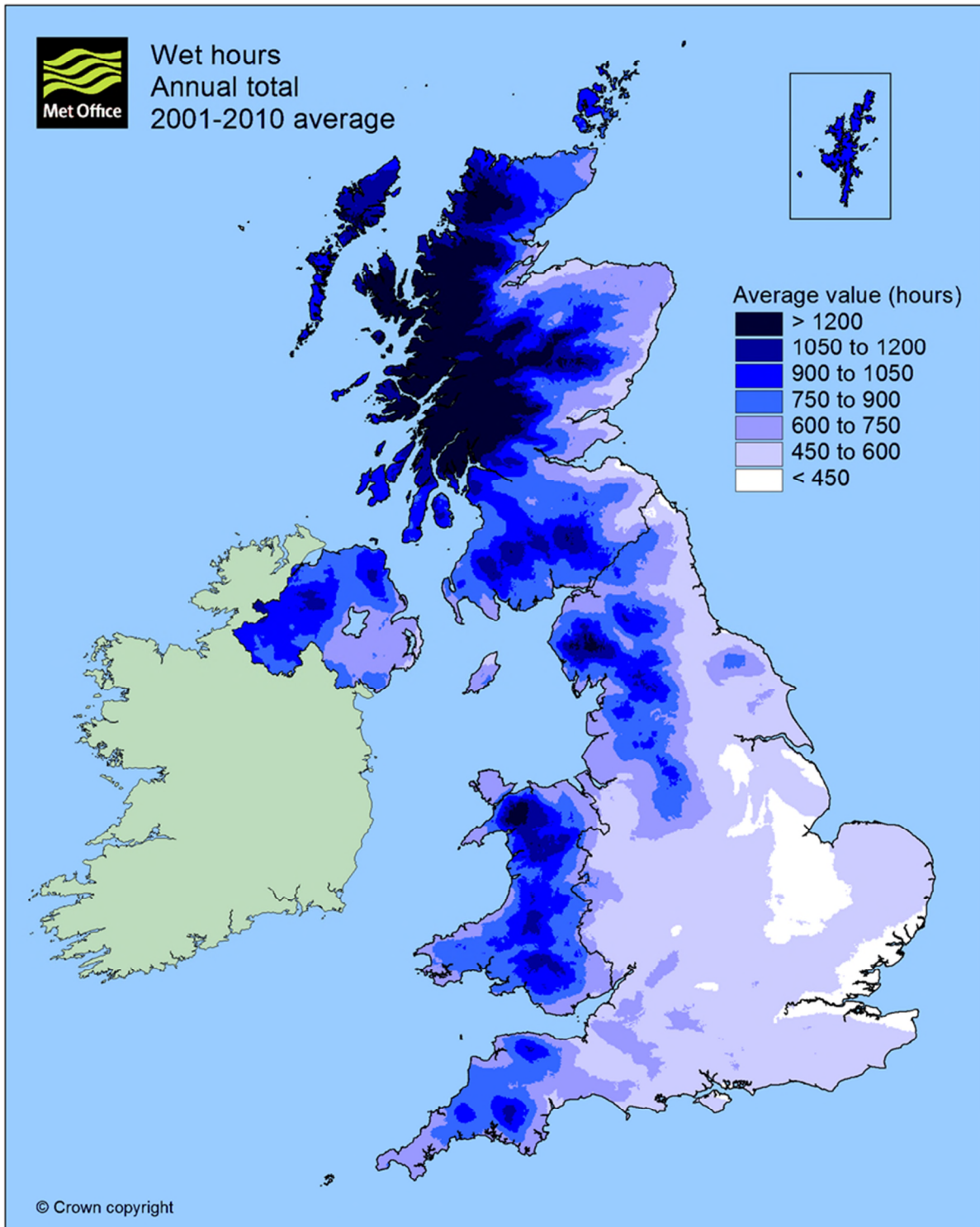
Figure 11D.2 Annual Average Wet Hours (above 0.2mm/hr), 2001-2010
