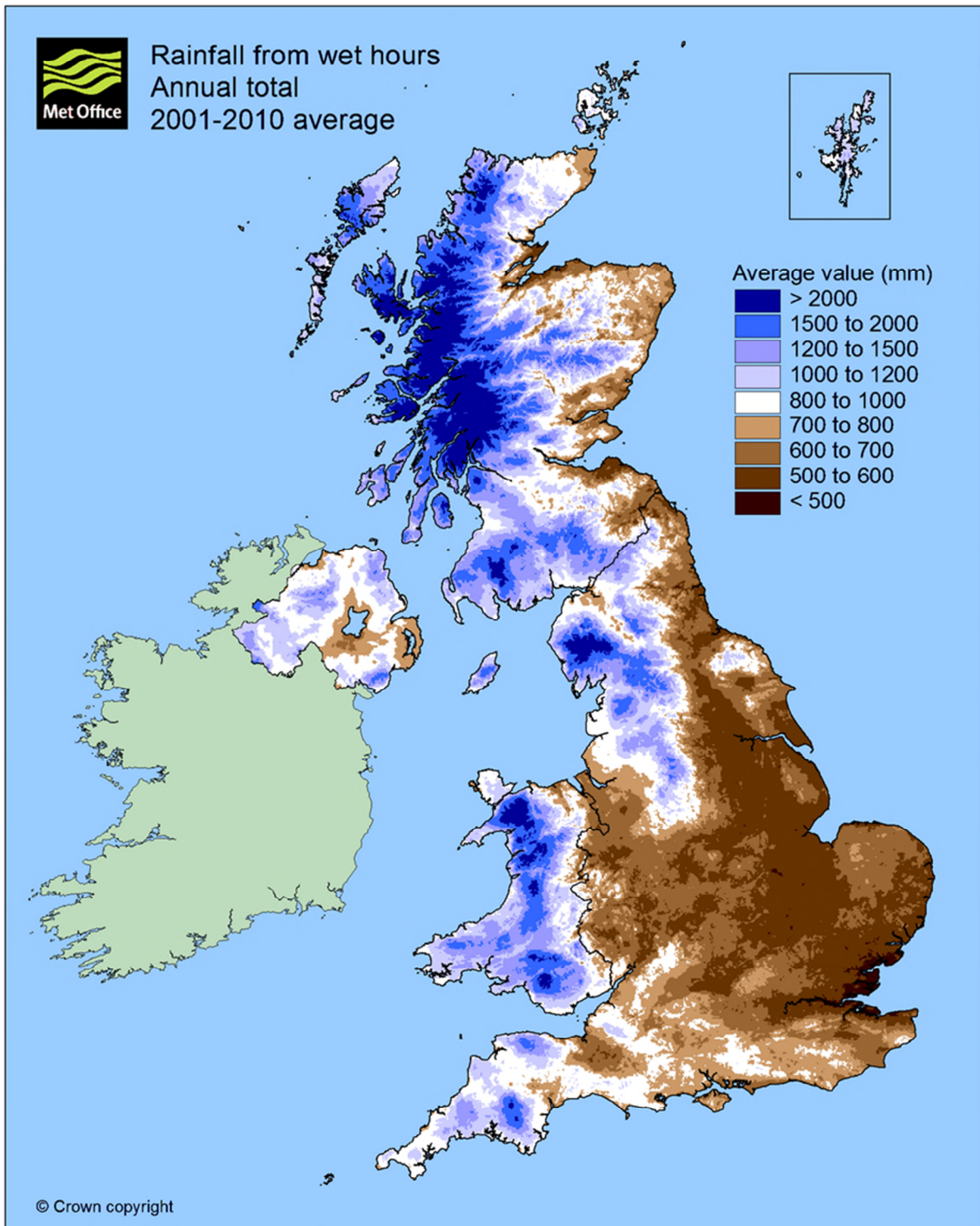
Figure 11D.1 Total annual average rainfall, 2001-2010
