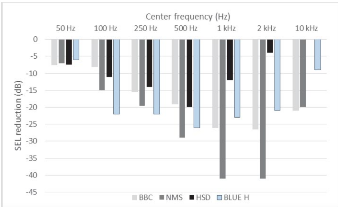
Figure 2: Reduction in SEL at the frequencies 100 Hz, 250 Hz, 500 Hz, 1 kHz and 2 kHz in the 1/3rd octave band frequency spectrum of a pile strike when comparing mitigated versus unmitigated piling (Verfuss et al. 2019).
