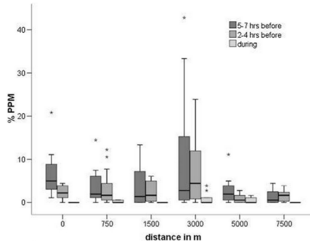
Figure 3: Percentage of porpoise positive minutes recorded before and during Lofitech trials at various distances (Brandt et al. 2013b).
