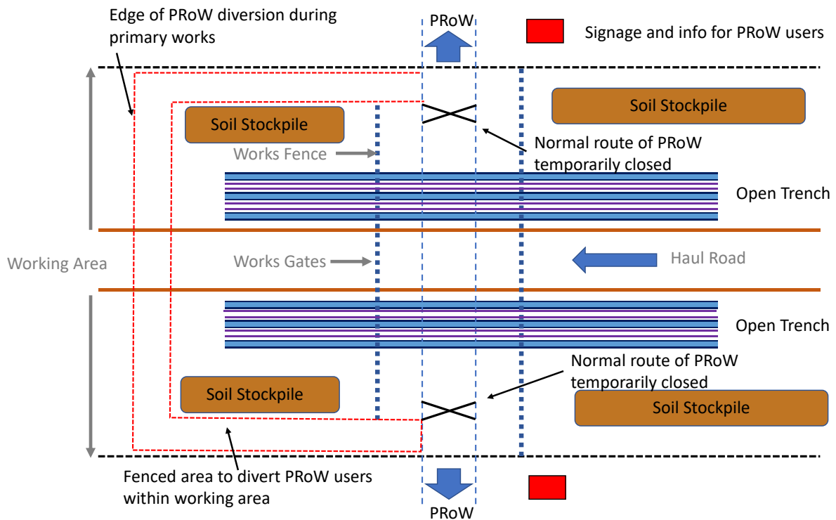
Figure 2: Indicative management of a short diversion to a PRow crossing the cable corridor during construction.
