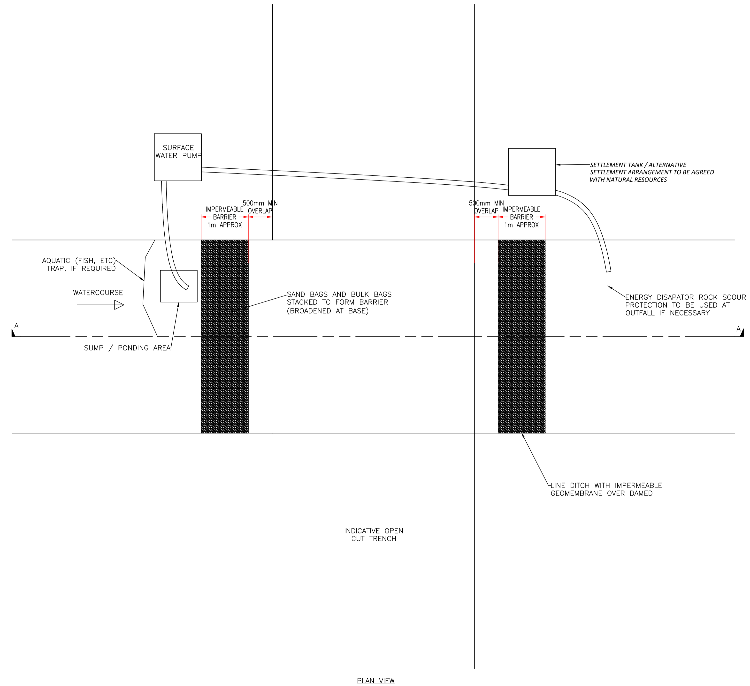
PLAN VIEW
