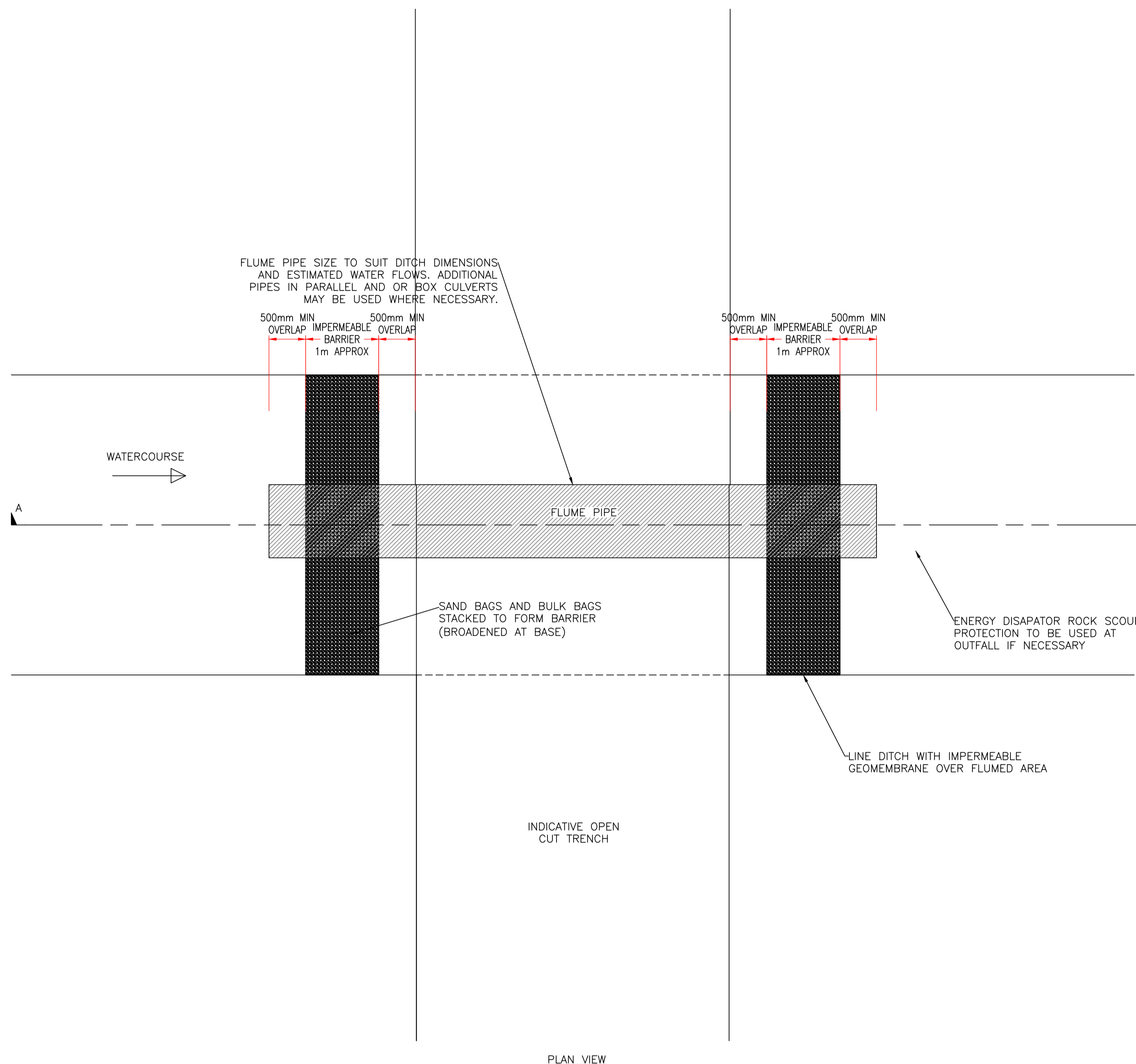
PLAN VIEW
