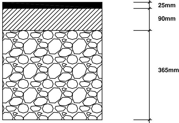
Type C: Heavy vehicle crossing footway/ cycleway
