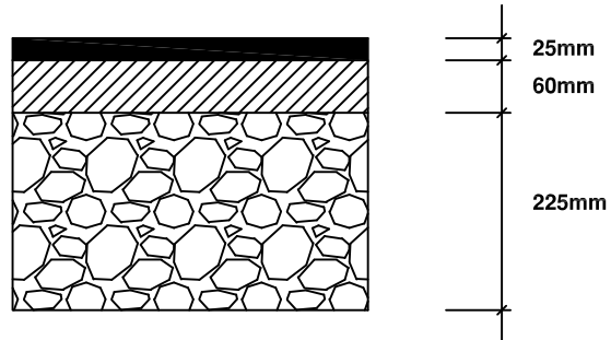
Type B: Footway/ cycleway or light vehicle crossing
