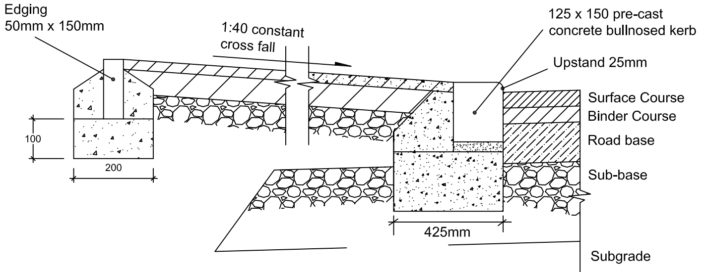
TYPICAL SECTION
