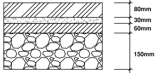
Type D: Footway (pedestrians only)
