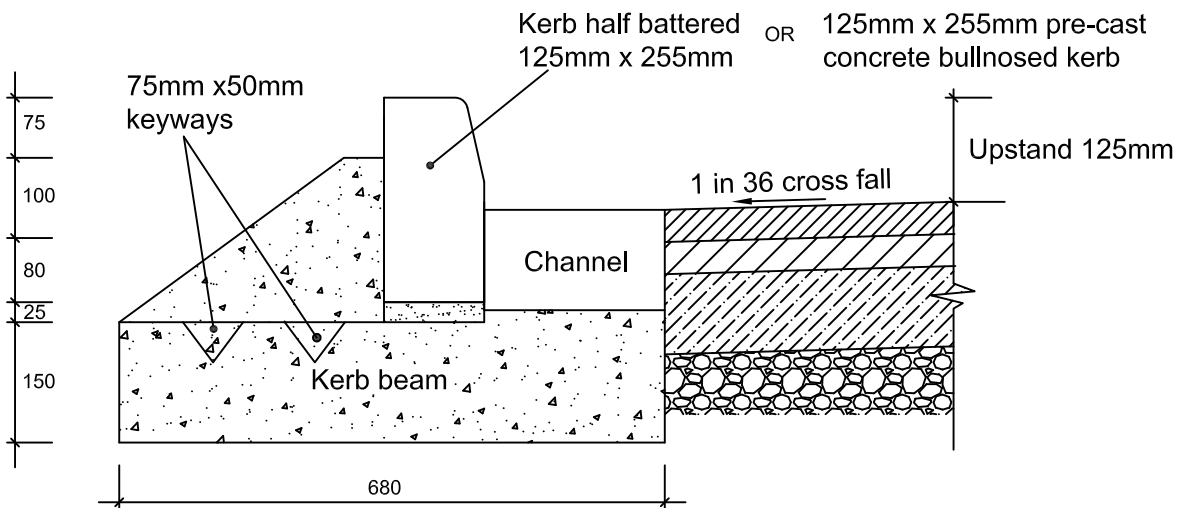
CHANNEL DETAIL
