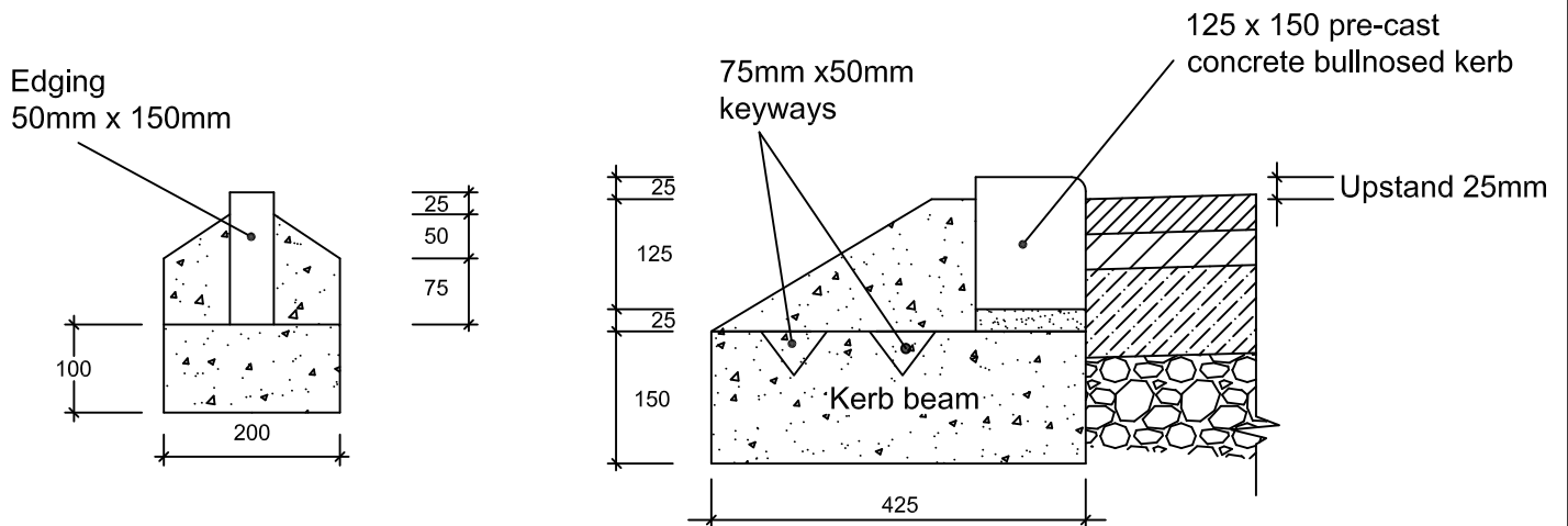
EDGING DETAIL
