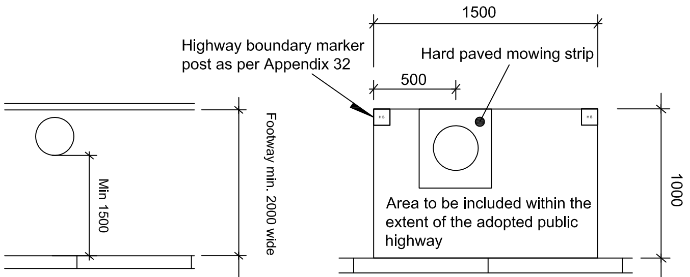
Location of Lighting Column within a footway
