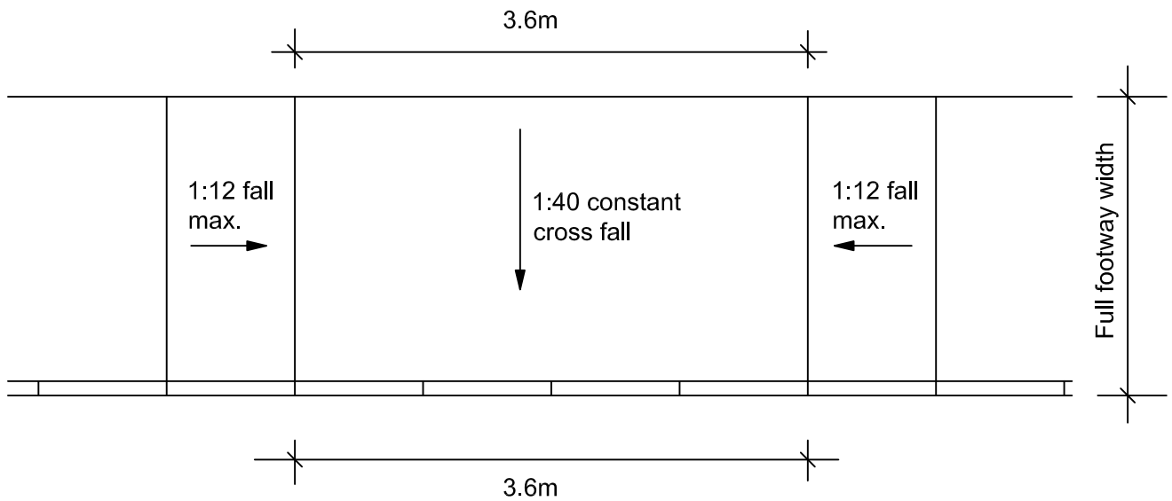
TYPICAL PLAN
