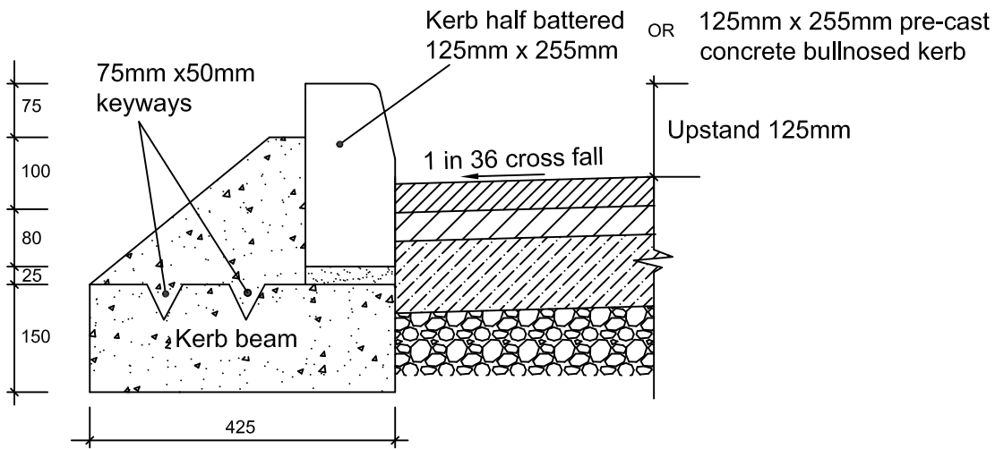
KERB DETAIL
