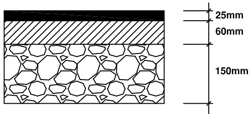
Type A: Footpath separate from carriageway (pedestrians only)
