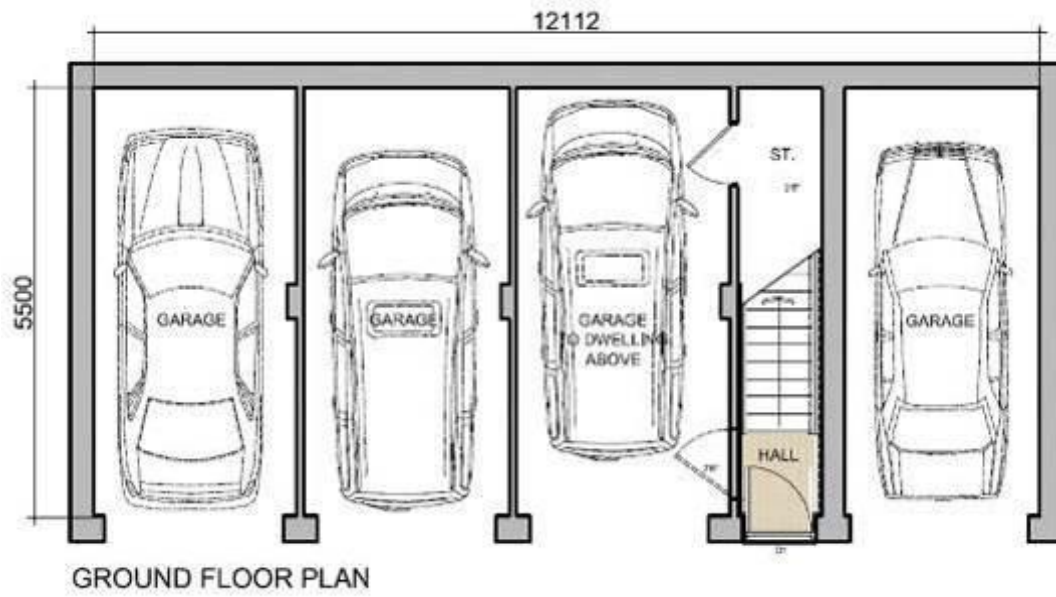
Unacceptable plan where one cannot open the car doors
