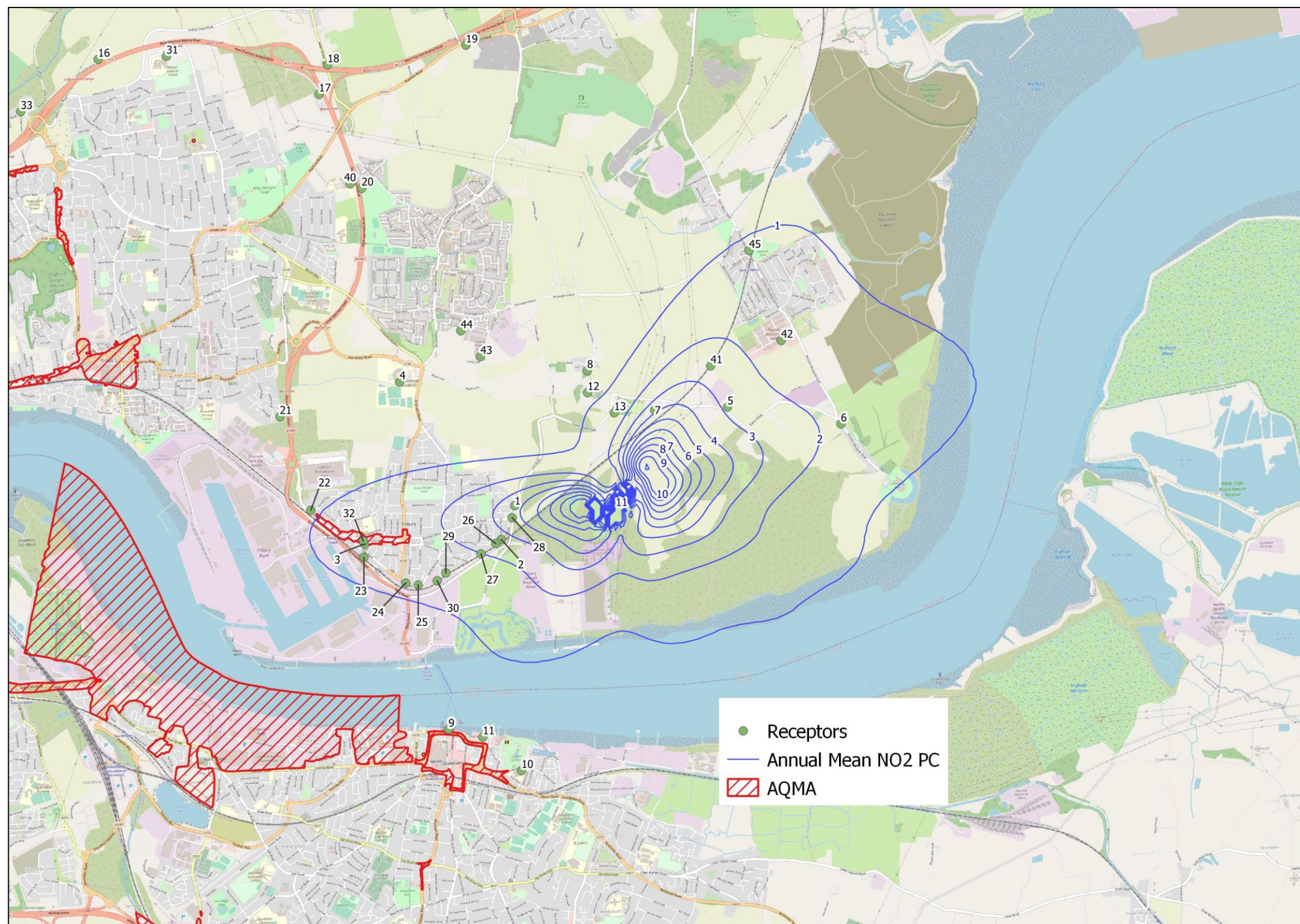
Figure 2: Annual Mean NO 2 Process Contributions ( \mu\text{g.m}^{-3} )
