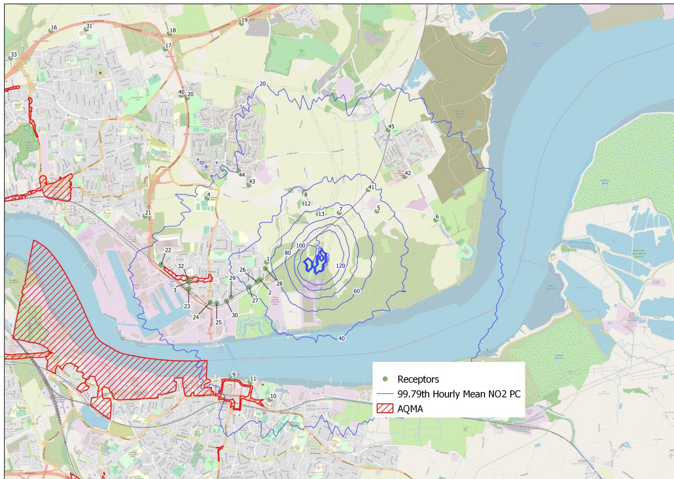
Figure 1: Hourly Mean NO 2 Process Contributions (µg.m -3 )
