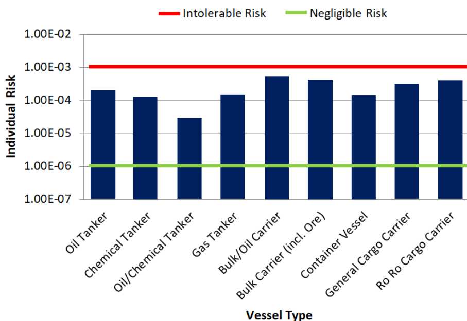
Figure 2.1 Individual Risk Levels and Acceptance Criteria per Vessel Type
