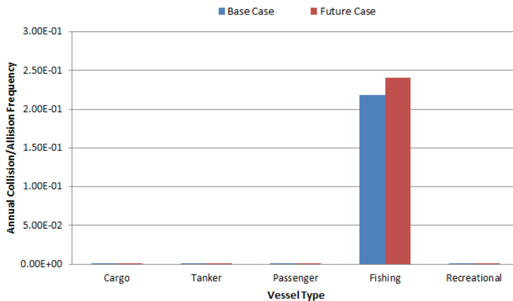
Figure 4.1 Change in Annual Collision and Allision Frequency by Vessel Type
