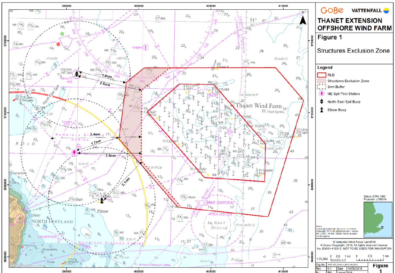
Figure 1. Thanet Extension Offshore Wind Farm (indicative layout).
