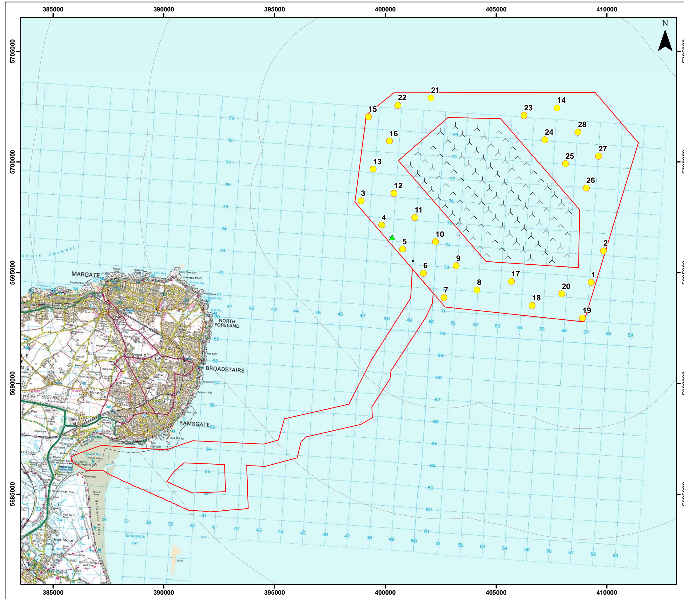
Figure 12.1a SLVIA Rochdale Envelope - 28 x 12MW Optimum Space Layout
