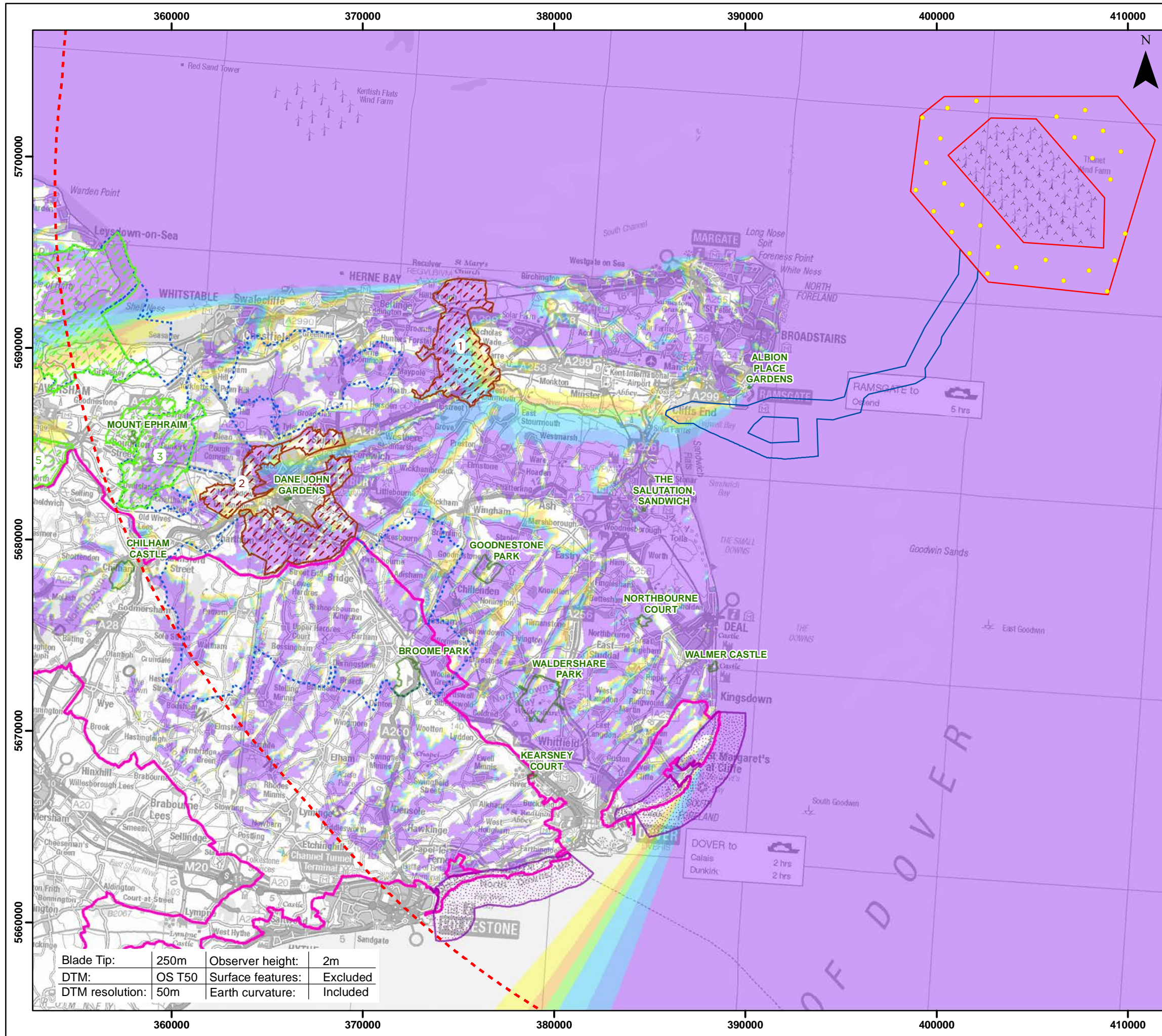
Figure 12.19 Blade Tip ZTV with Landscape Designations
