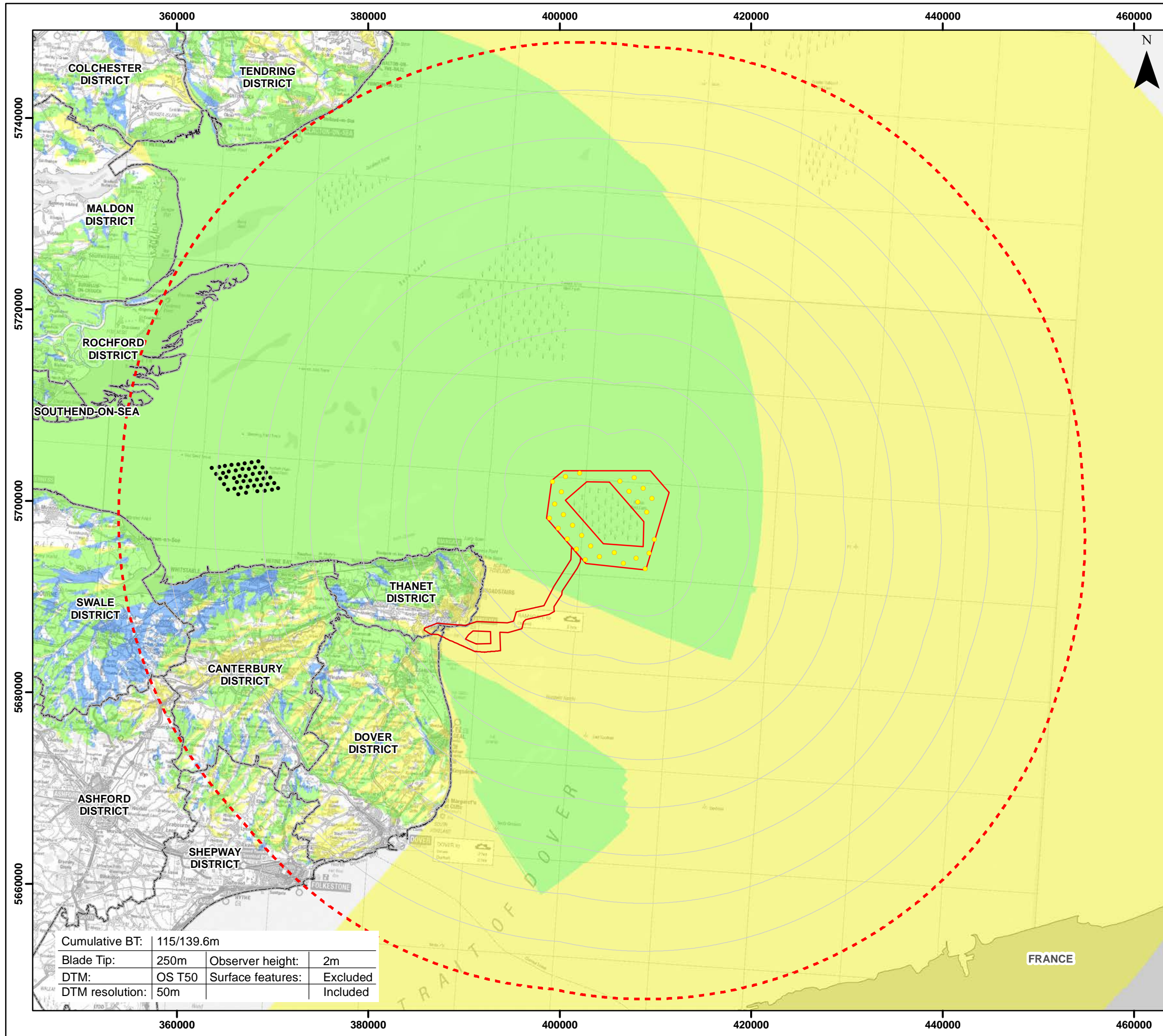
Figure 12.24 Cumulative ZTV - Kentish Flats & Extension
