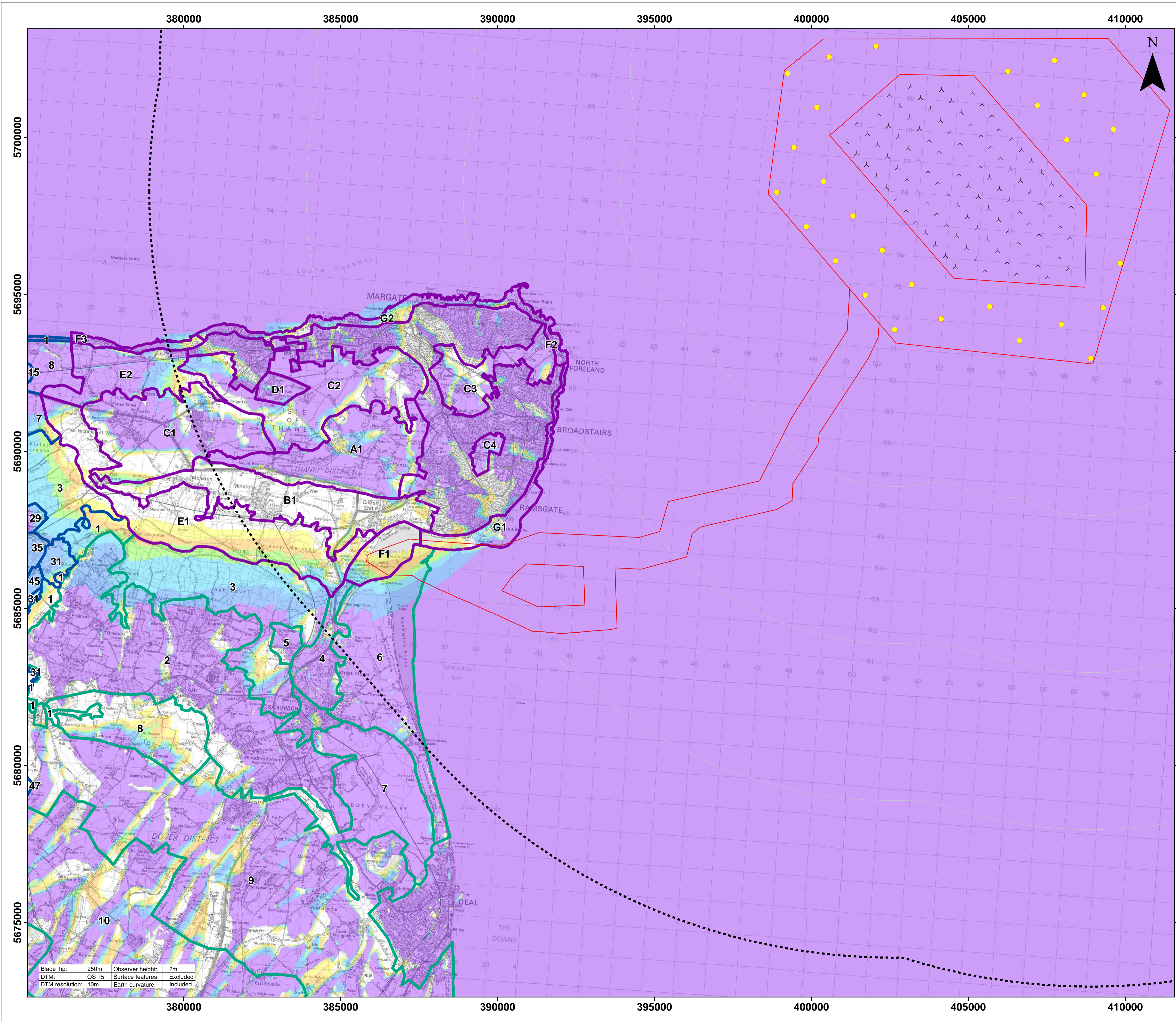
Figure 12.17 Blade Tip ZTV with Landscape Character (District) - 20km
