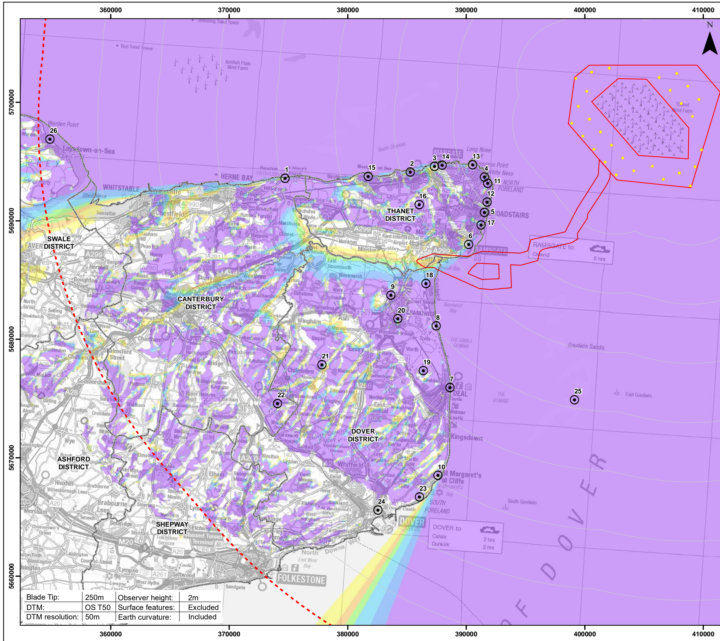
Figure 12.6 Blade Tip ZTV - Kent
