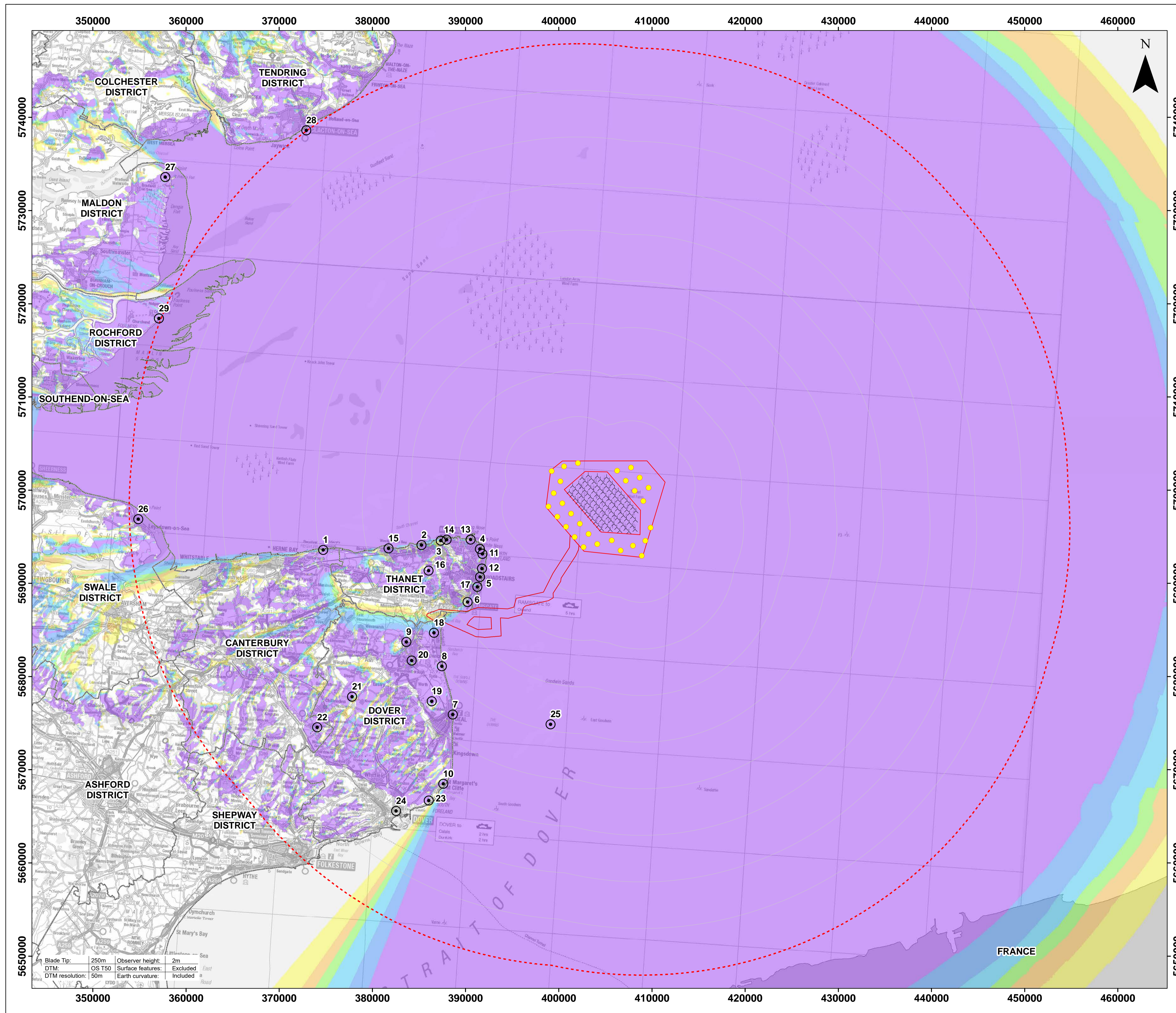
Figure 12.5 Blade Tip ZTV - 45km Study Area
