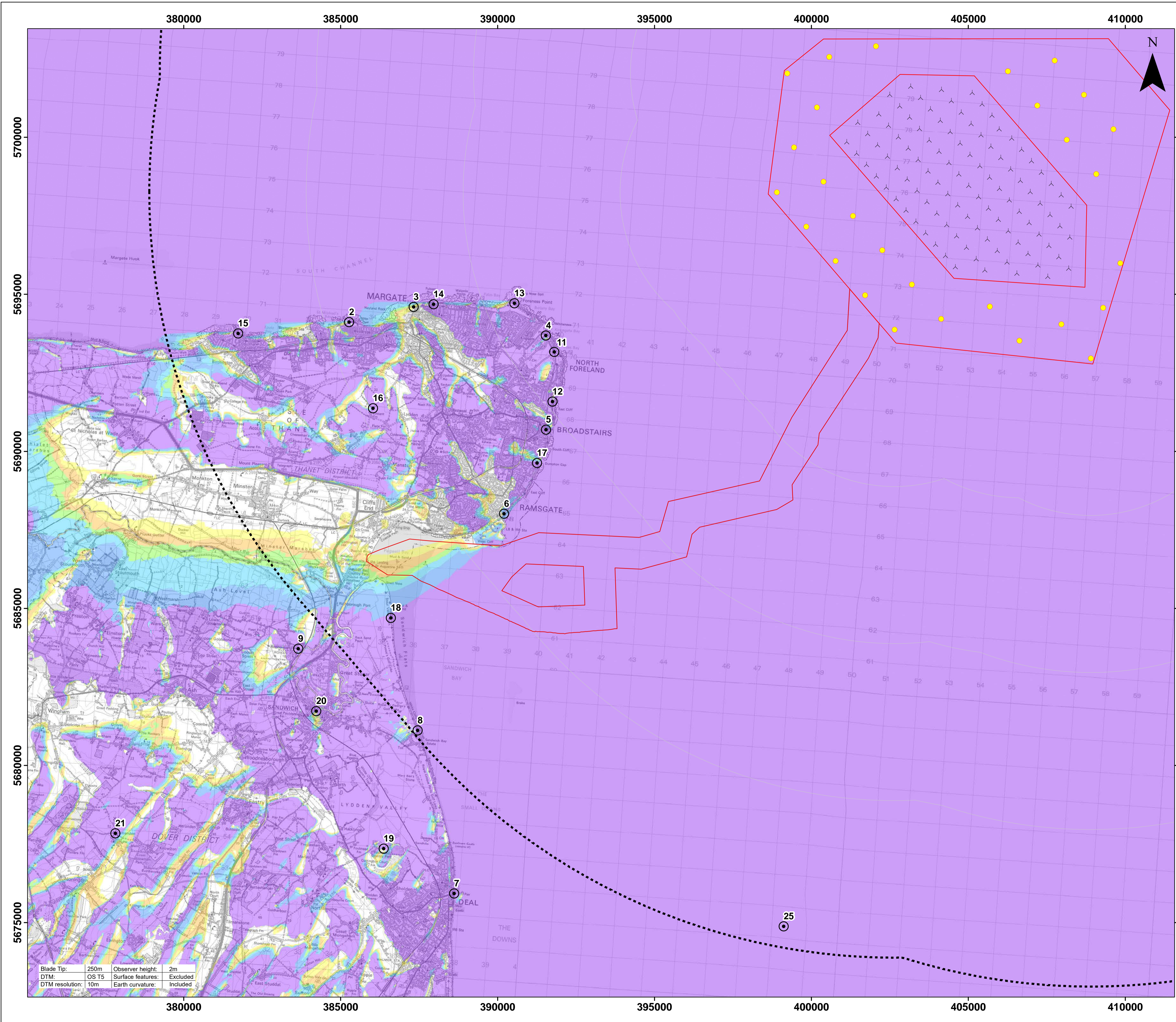
Figure 12.8 Blade Tip ZTV - 20km
