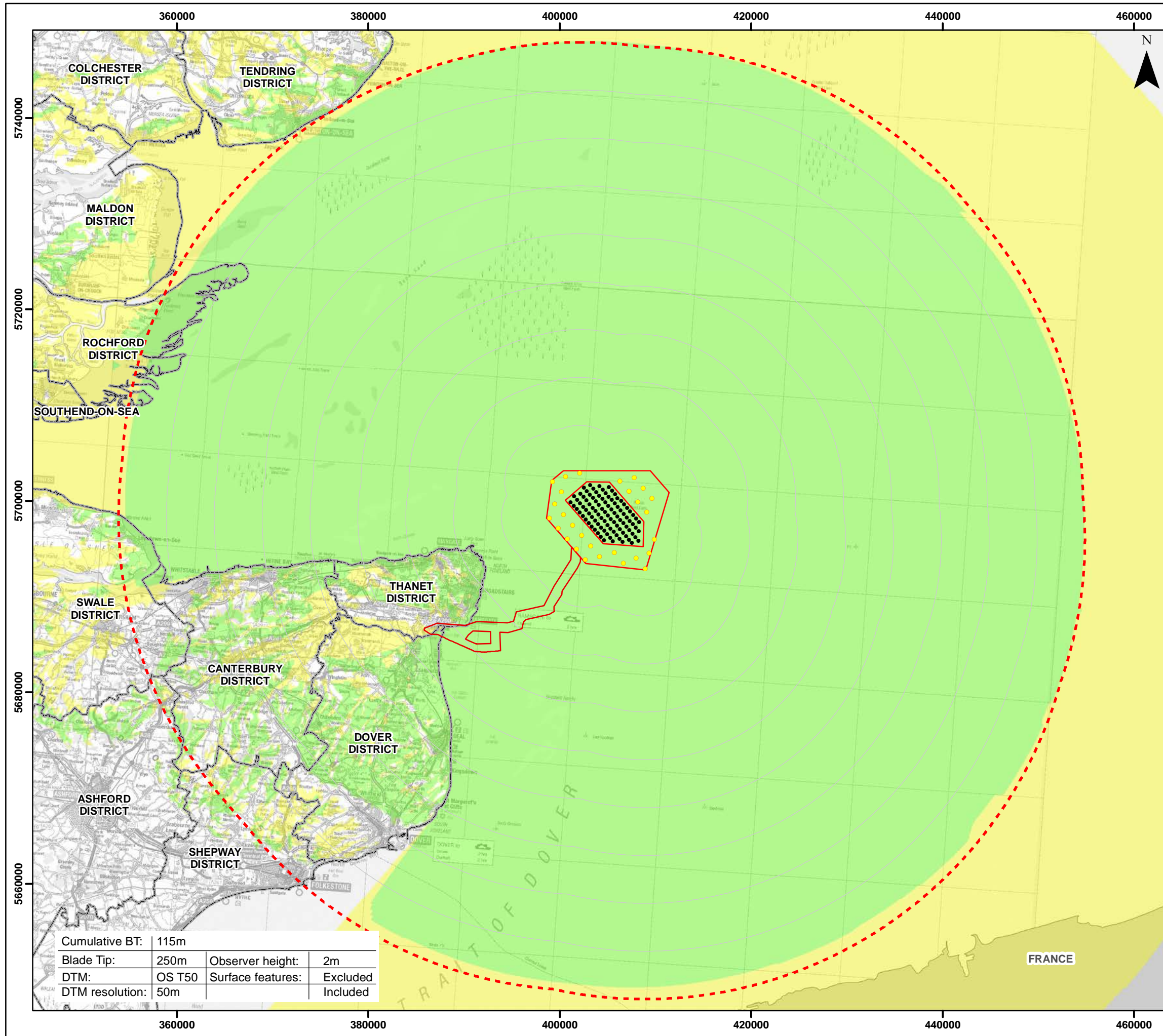
Figure 12.22 Cumulative ZTV - Thanet Offshore Wind Farm
