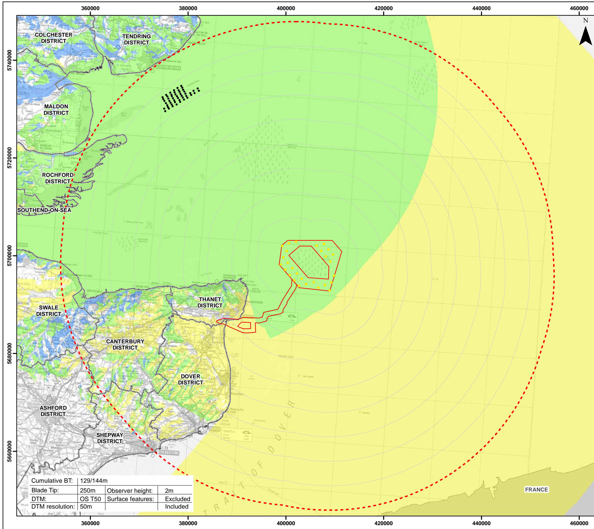
Figure 12.25 Cumulative ZTV - Gunfleet Sands I/II/III
