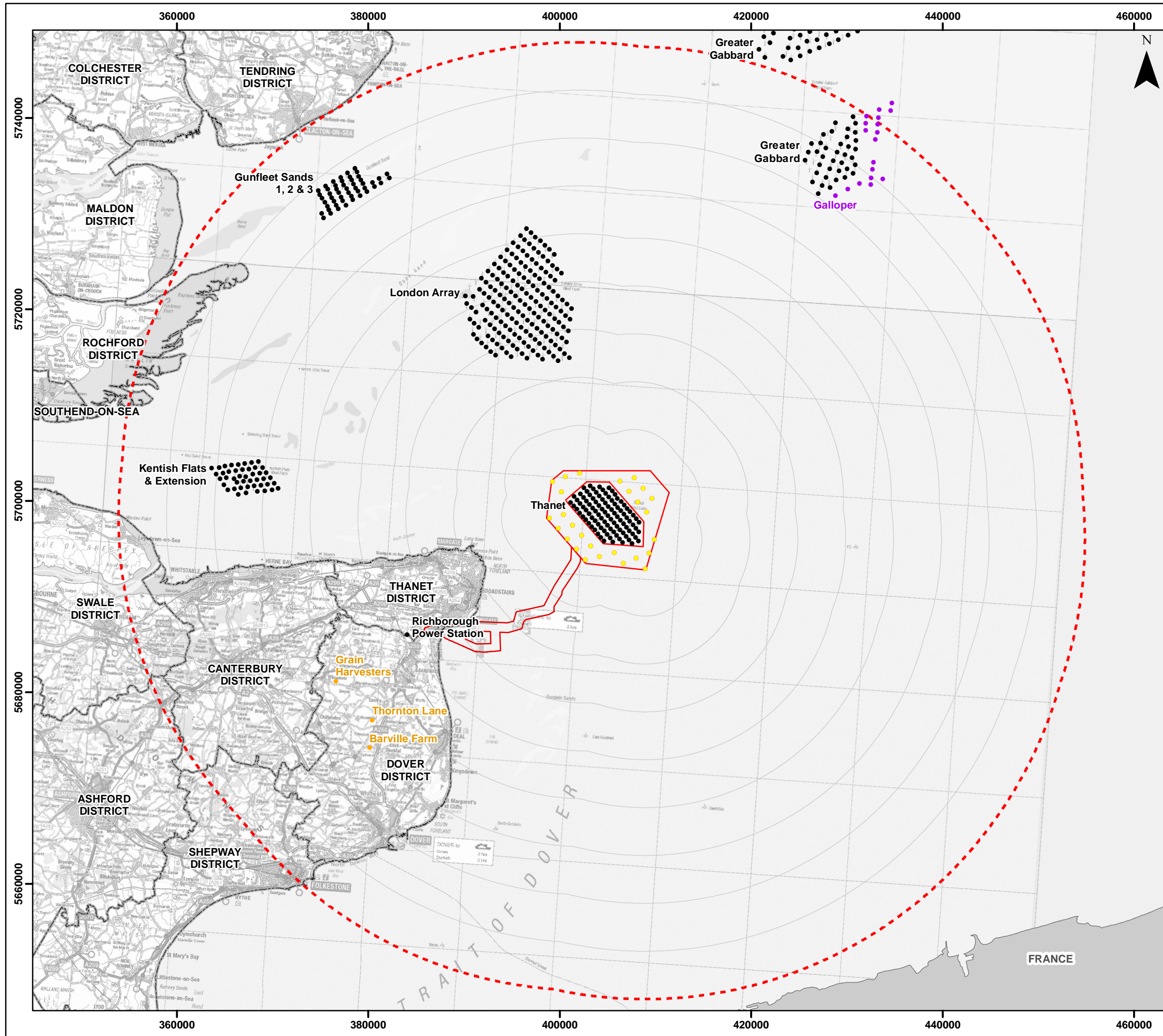
Figure 12.11 Other Wind Energy Developments
