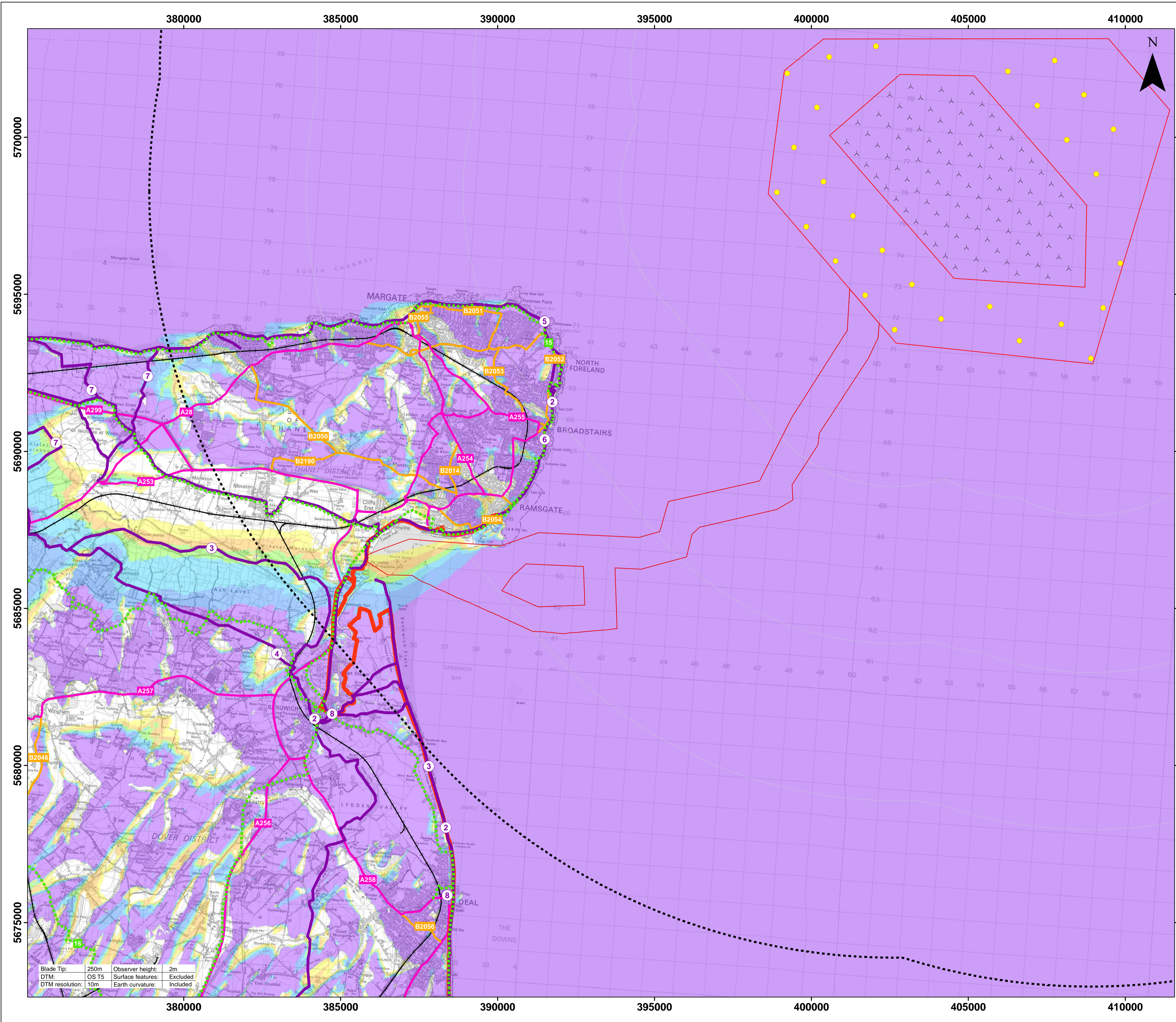
Figure 12.21 Blade Tip ZTV with Visual Receptors - 20km
