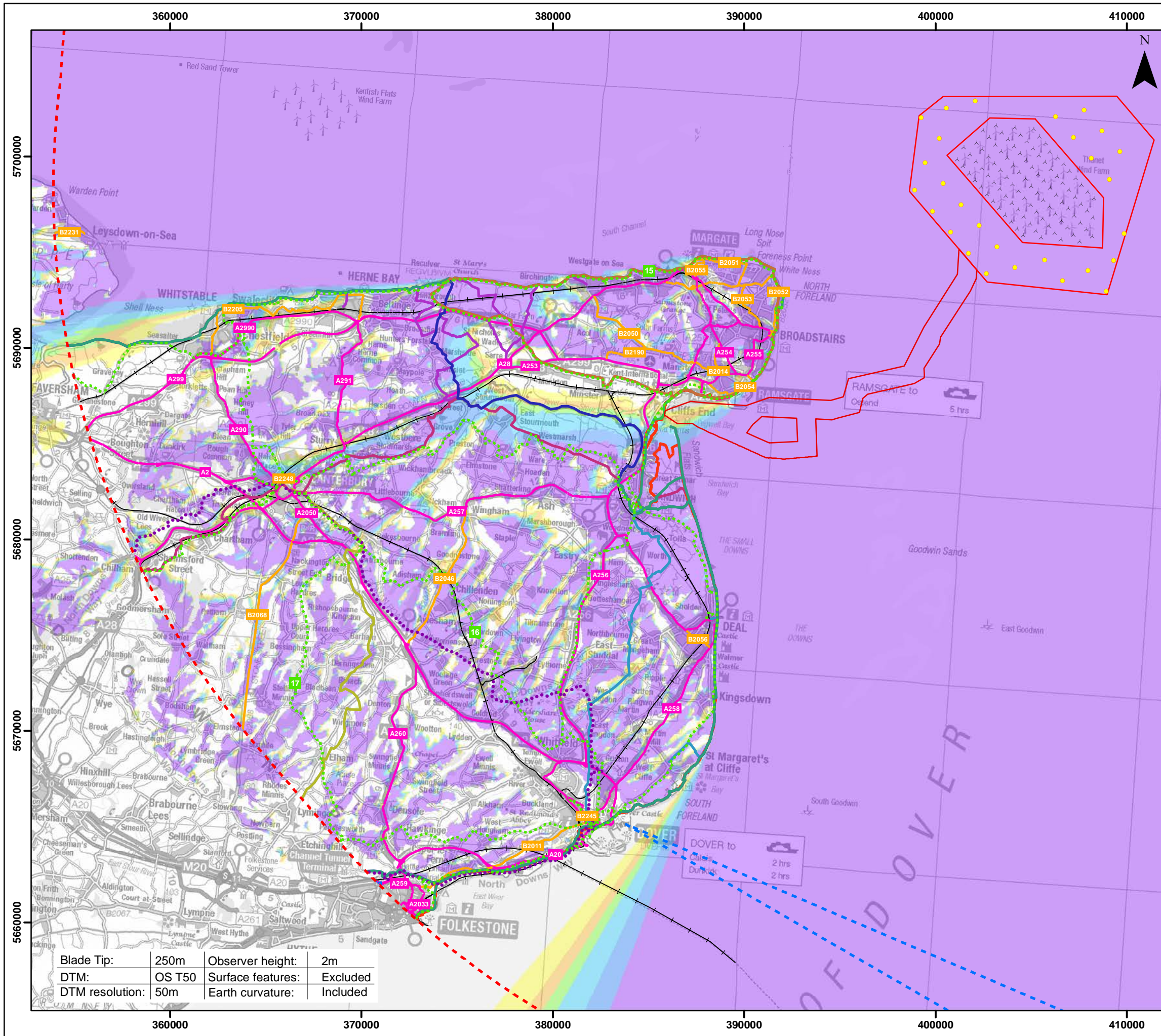
Figure 12.20 Blade Tip ZTV with Visual Receptors
