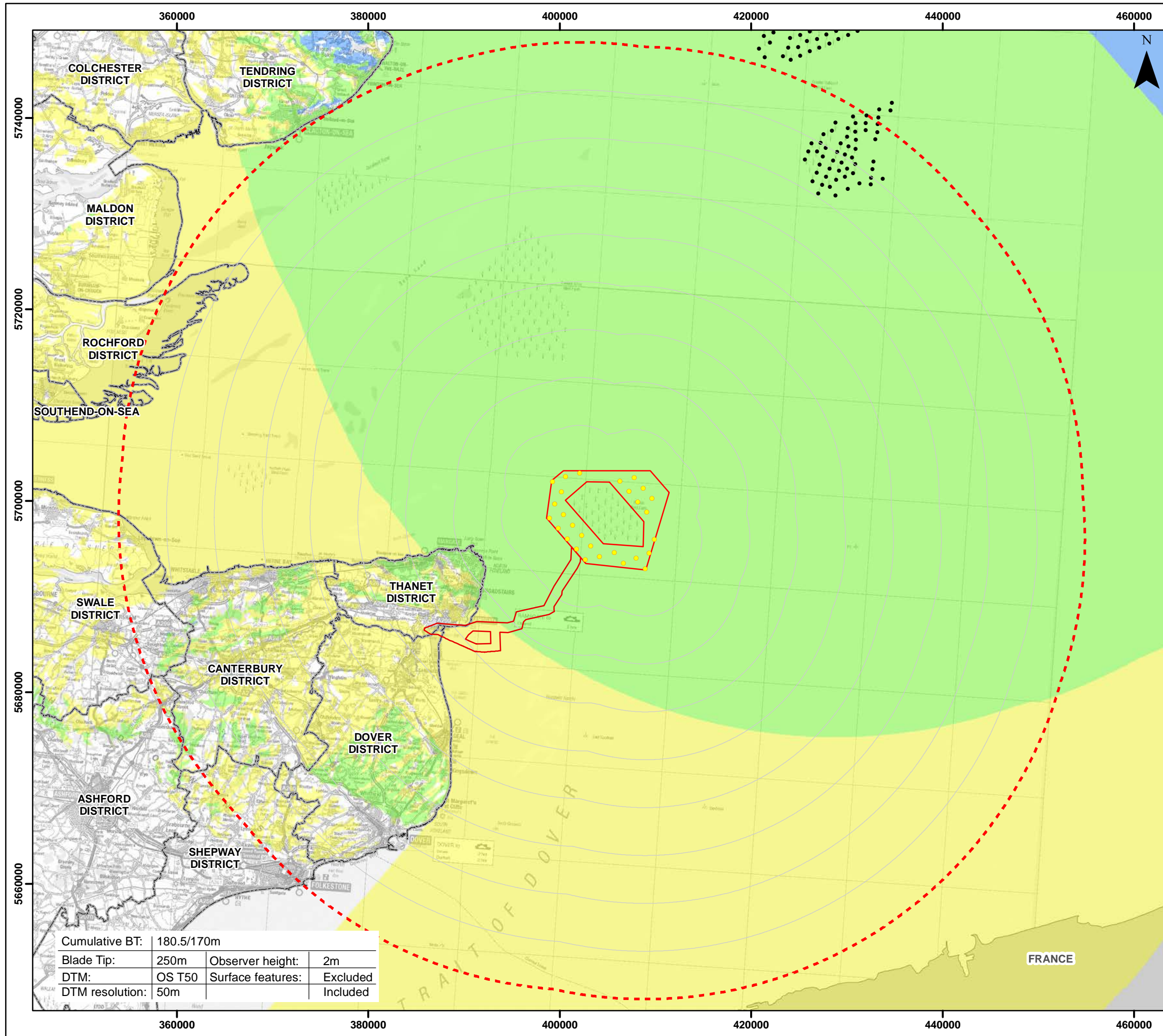
Figure 12.26 Cumulative ZTV - Greater Gabbard & Galloper
