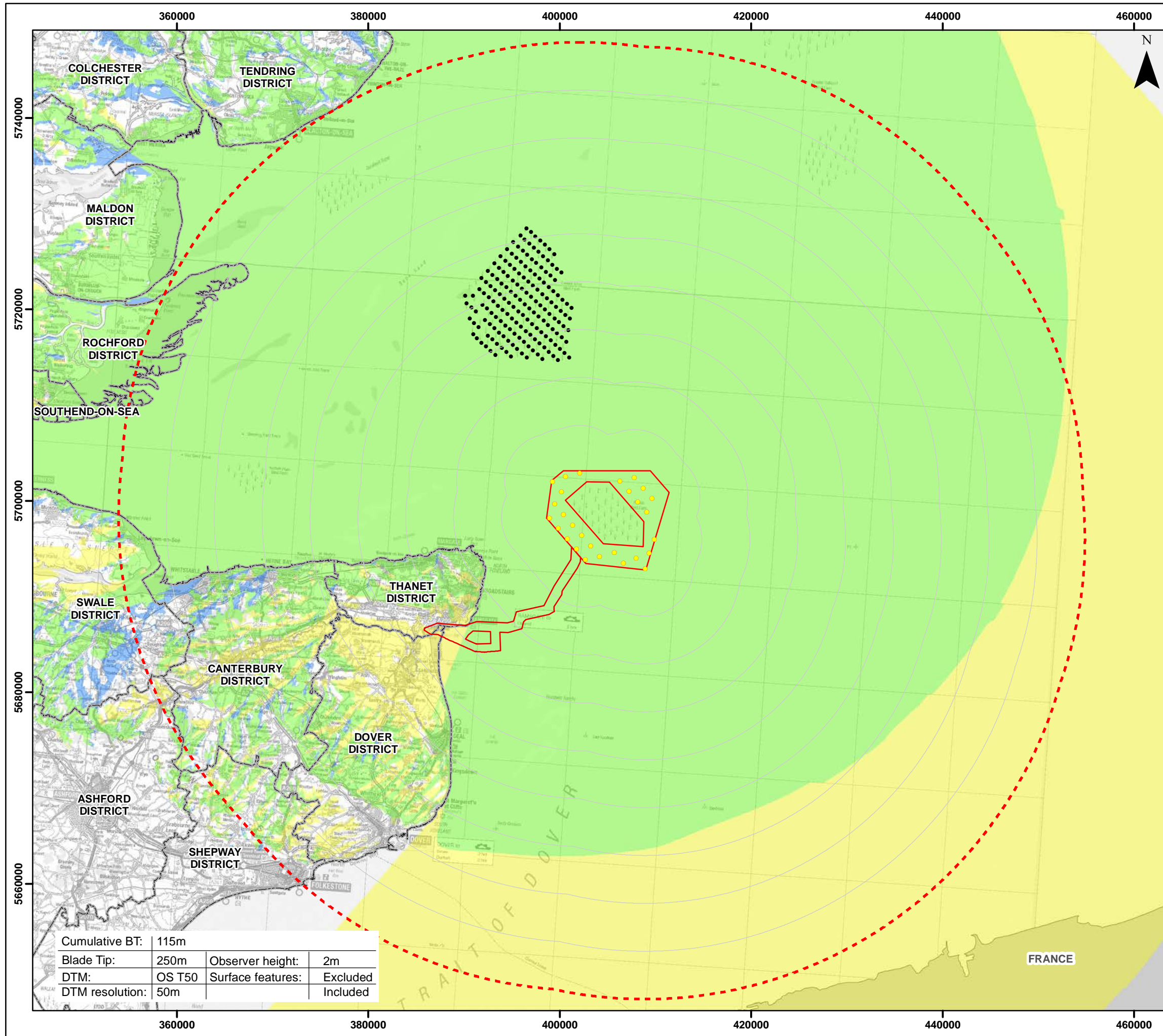
Figure 12.23 Cumulative ZTV - London Array
