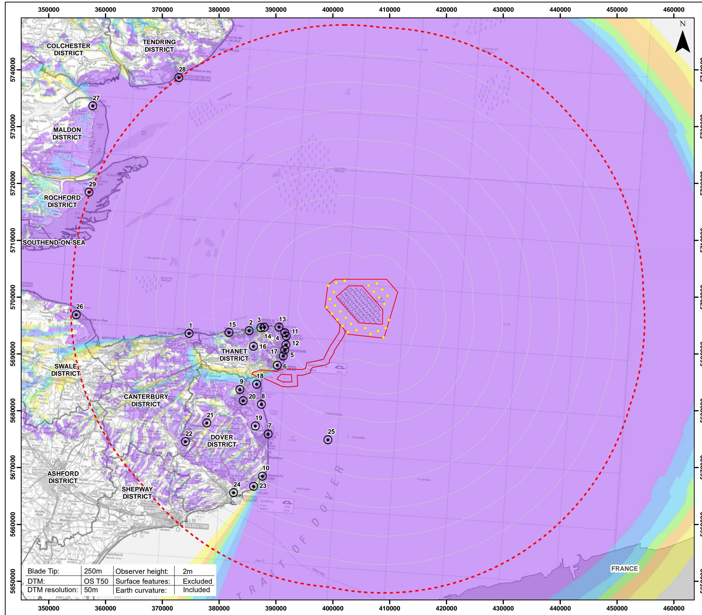
Figure 12.4 Blade Tip ZTV - 45km Study Area
