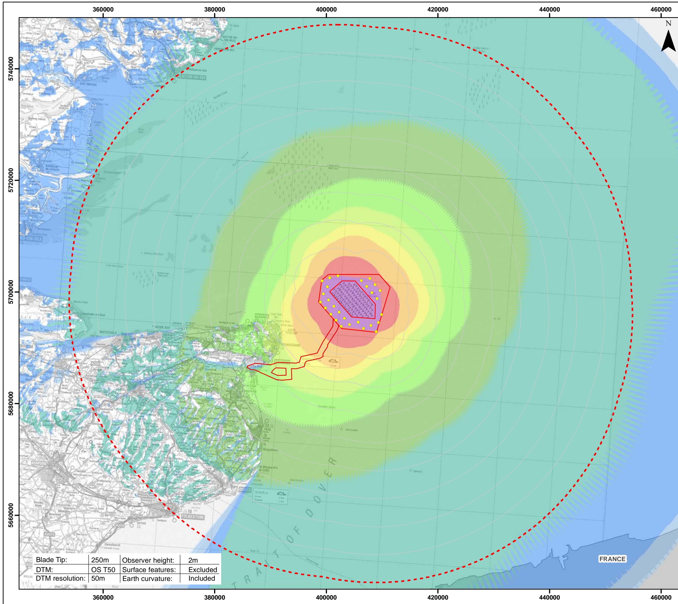
Figure 12.10 Horizontal Blade Tip ZTV
