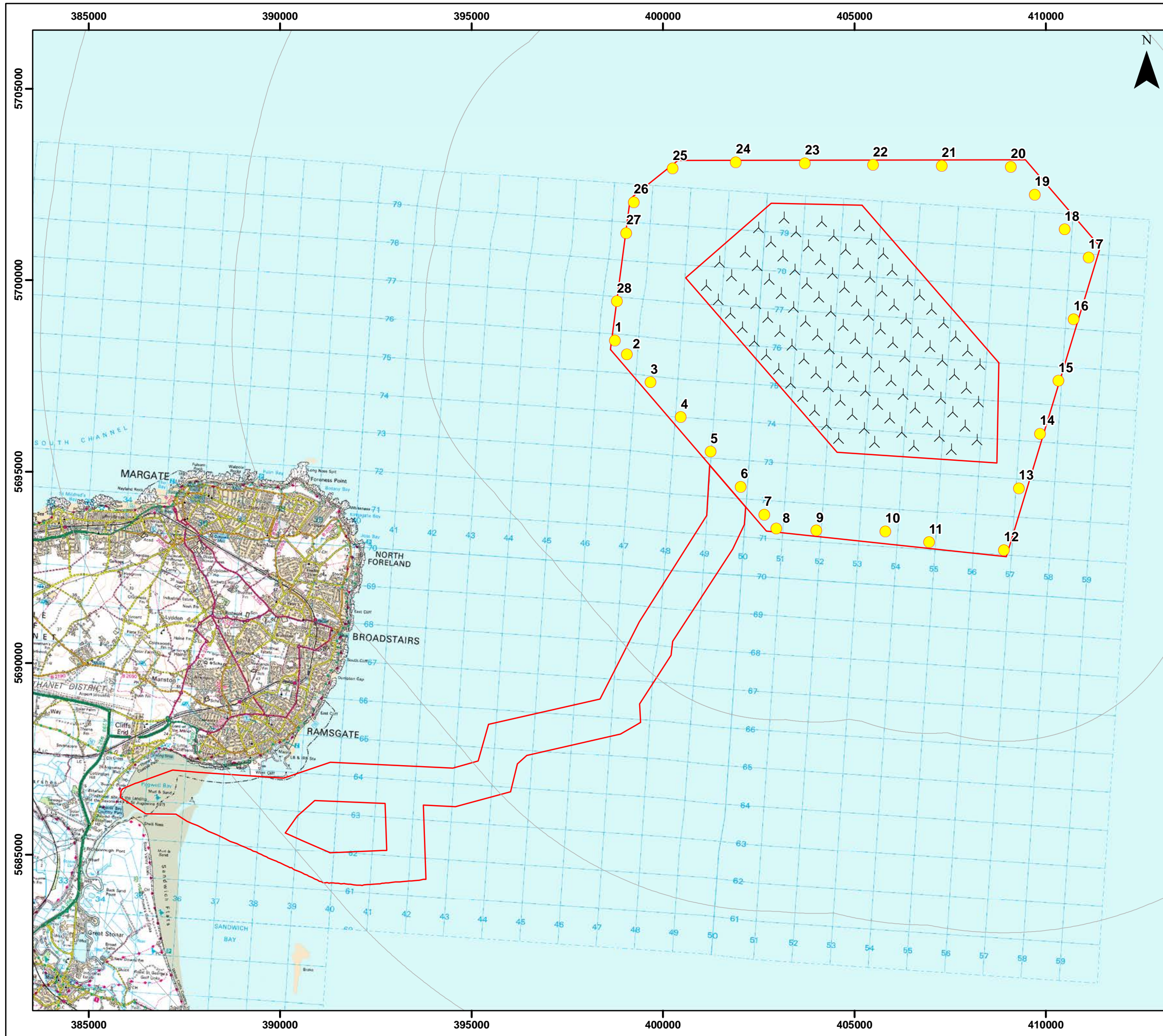
Figure 12.1b SLVIA Rochdale Envelope - 28 x 12MW Perimeter Layout
