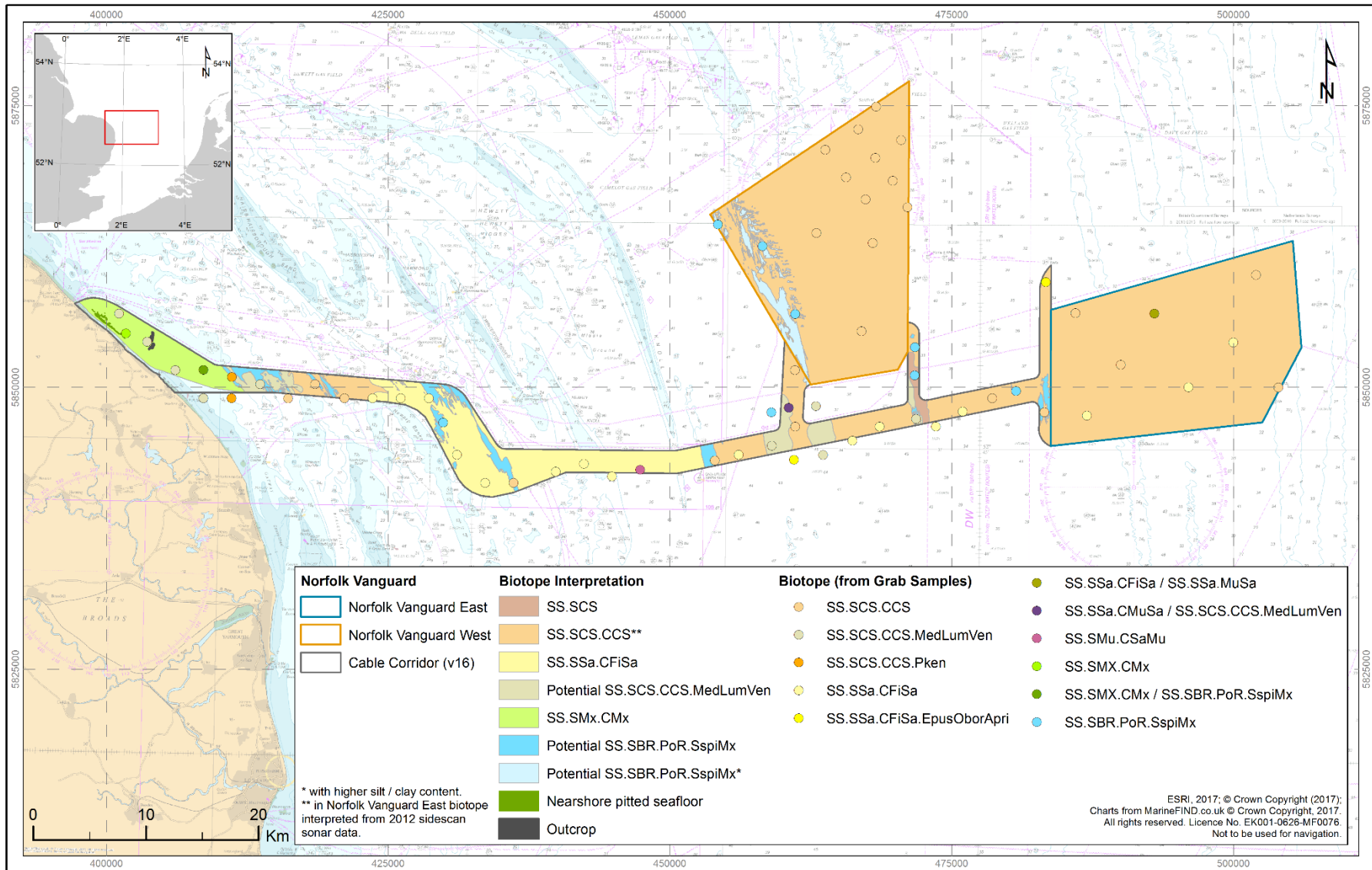
Figure 5.25 Biotopes in the survey area
