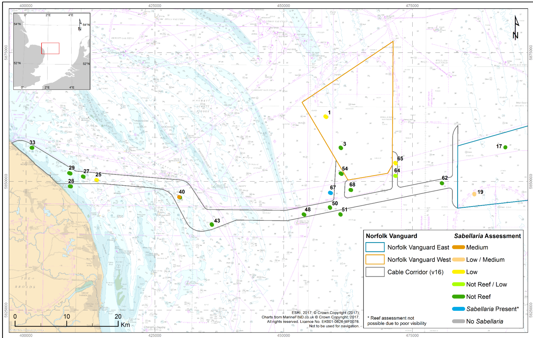
Figure 5.1 Sabellaria assessment across the survey area
