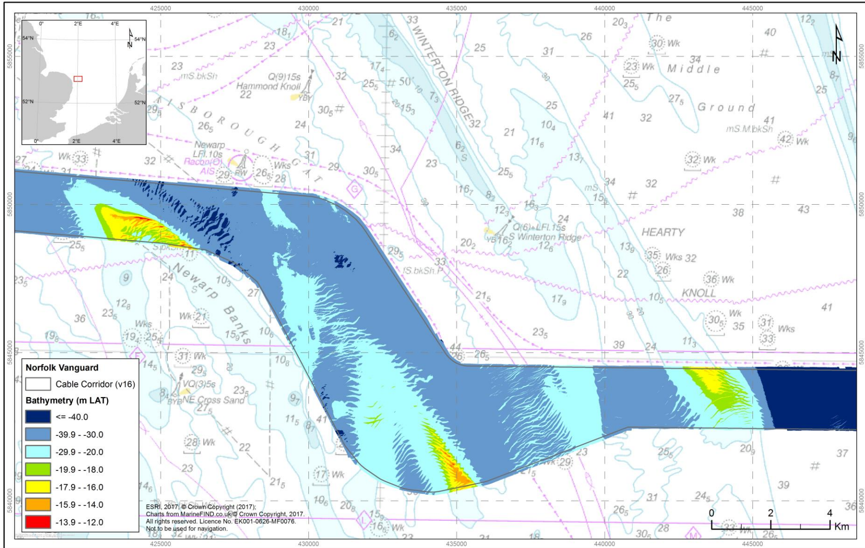
Figure 5.2 Sandbank assessment based on Topography
