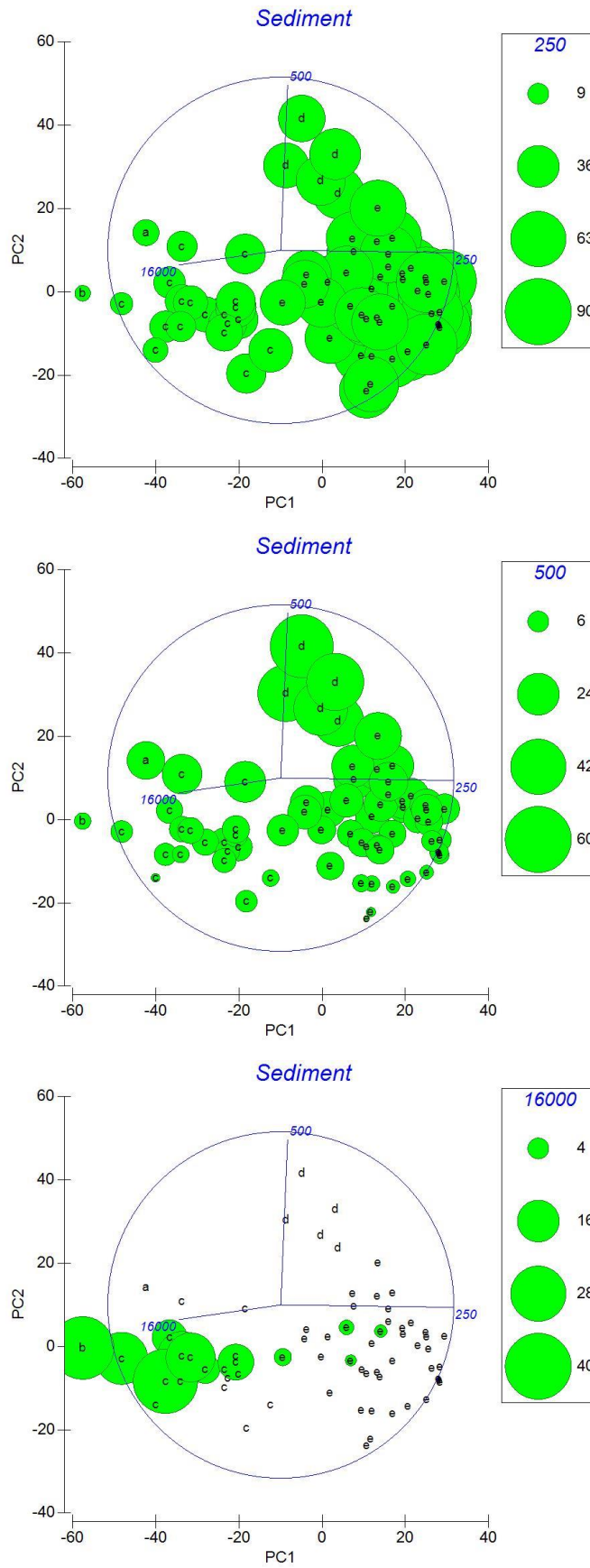
Figure 5.11: PCA ordination of particle sizes phi 2, 1 and -4 (% fine sand to coarser gravel) across the stations - the groups obtained by the multivariate analysis are overlaid
