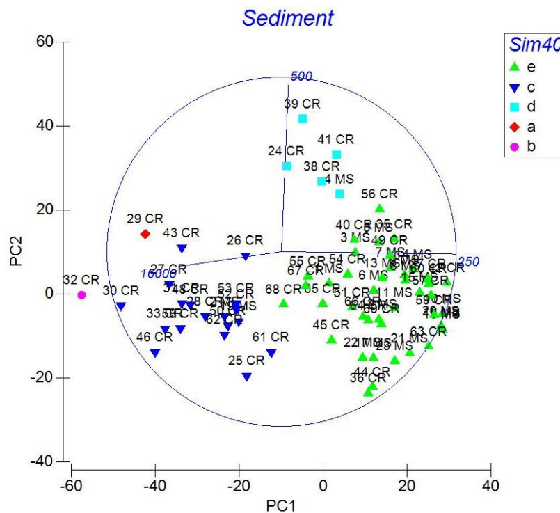
Figure 5.10: PCA ordination of particle sizes
