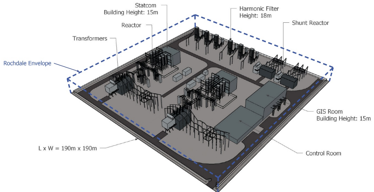
Plate A29.1 East Anglia TWO and East Anglia ONE North Onshore Substation Rochdale Envelope 3D Model
