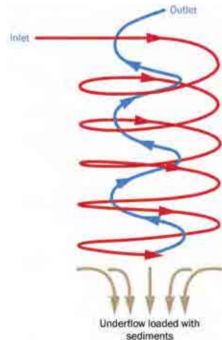
Figure 14.4 Simplified flow pattern in a vortex separator (from NJCAT, 2005)
