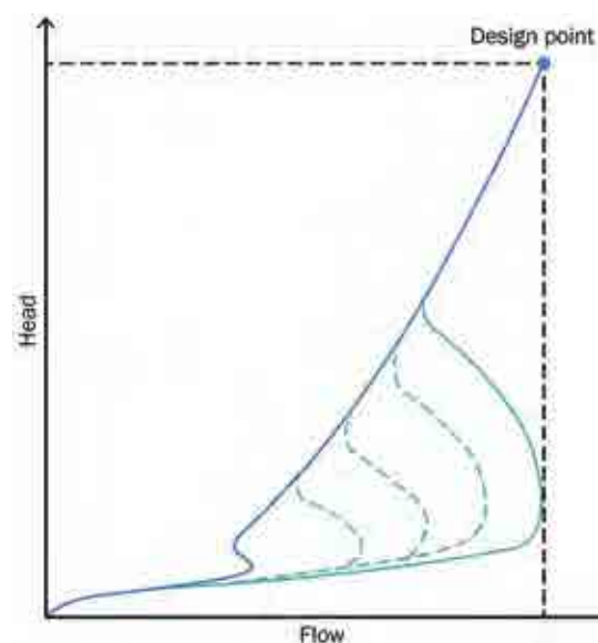
Figure 28.23 Examples of varying hydraulic performance for passive (vortex) type devices (courtesy Hydro International)
