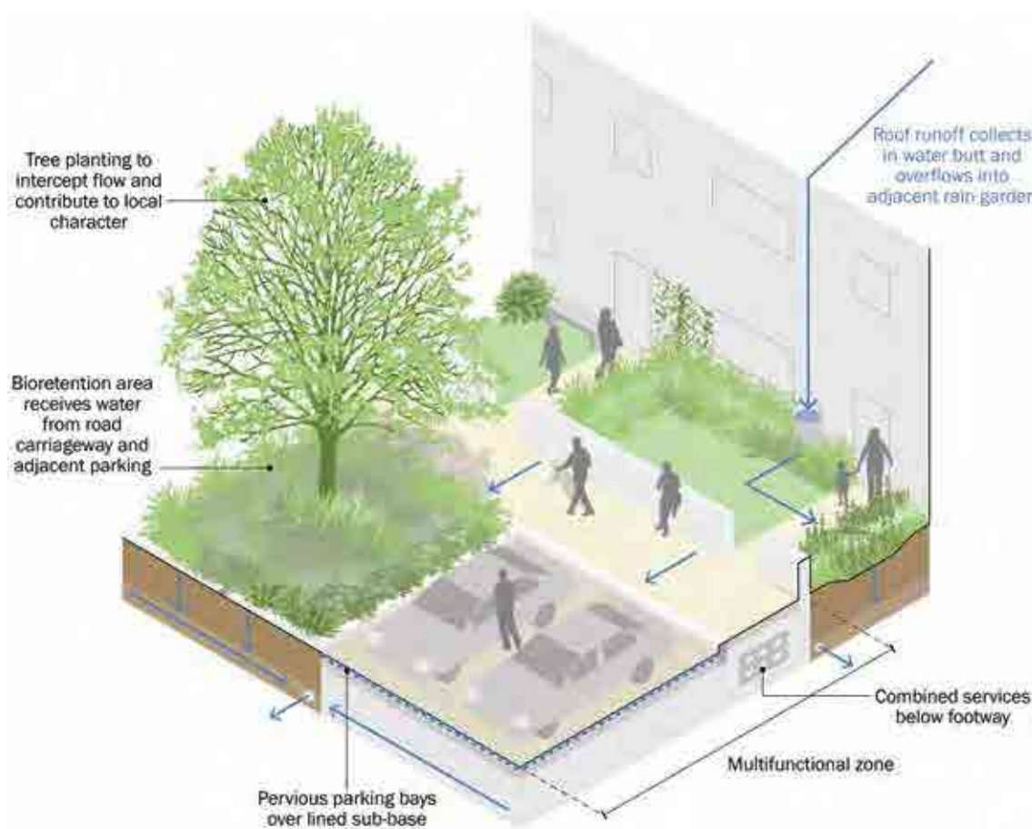
Figure 10.16 Multi-functional streetscape
