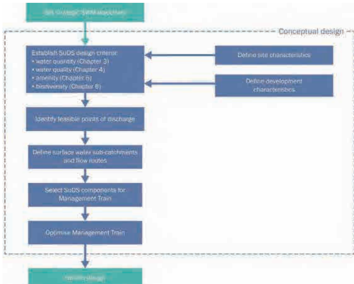
Figure 7.3 The conceptual design process
