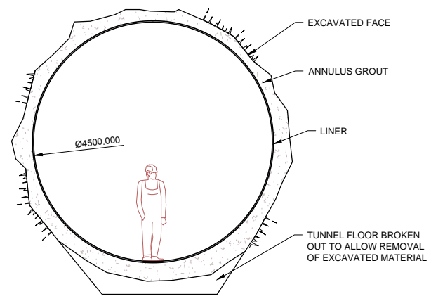
J | TYPICAL TUNNEL SECTION
