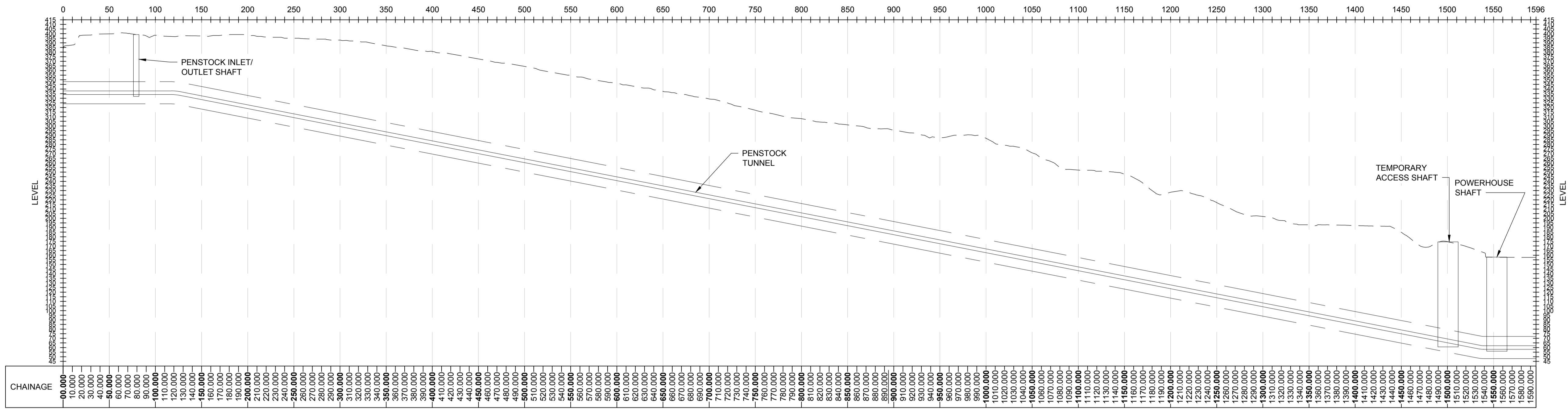
G | PENSTOCK TUNNEL SECTION
