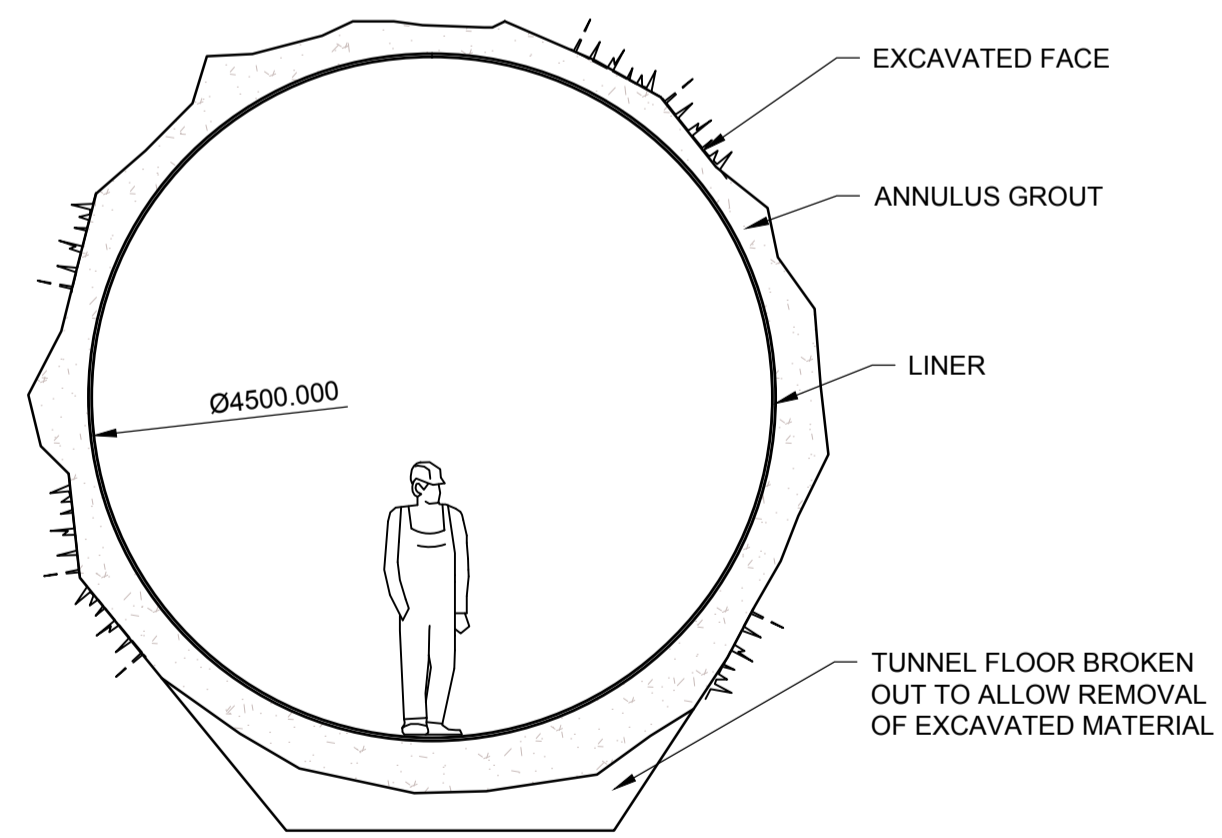
J | TYPICAL TUNNEL SECTION
