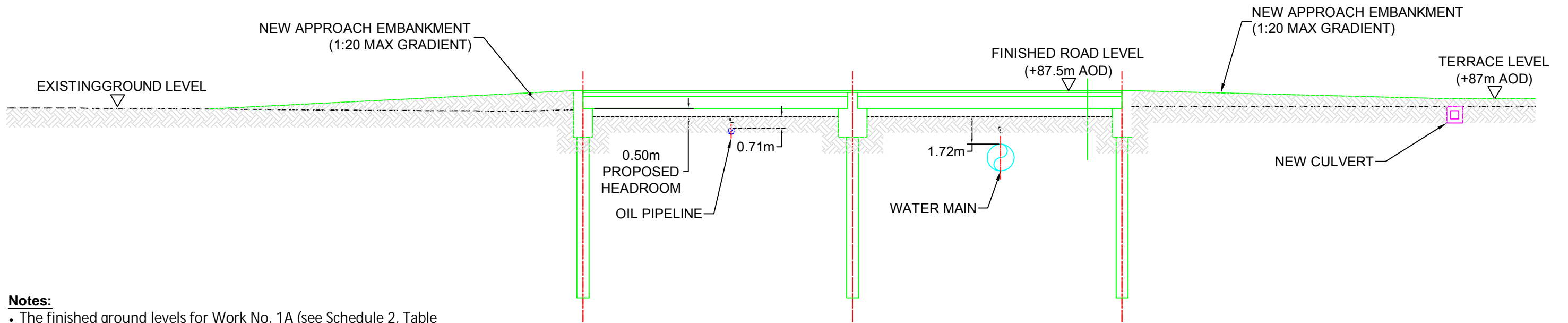
Long Section (Looking East)
