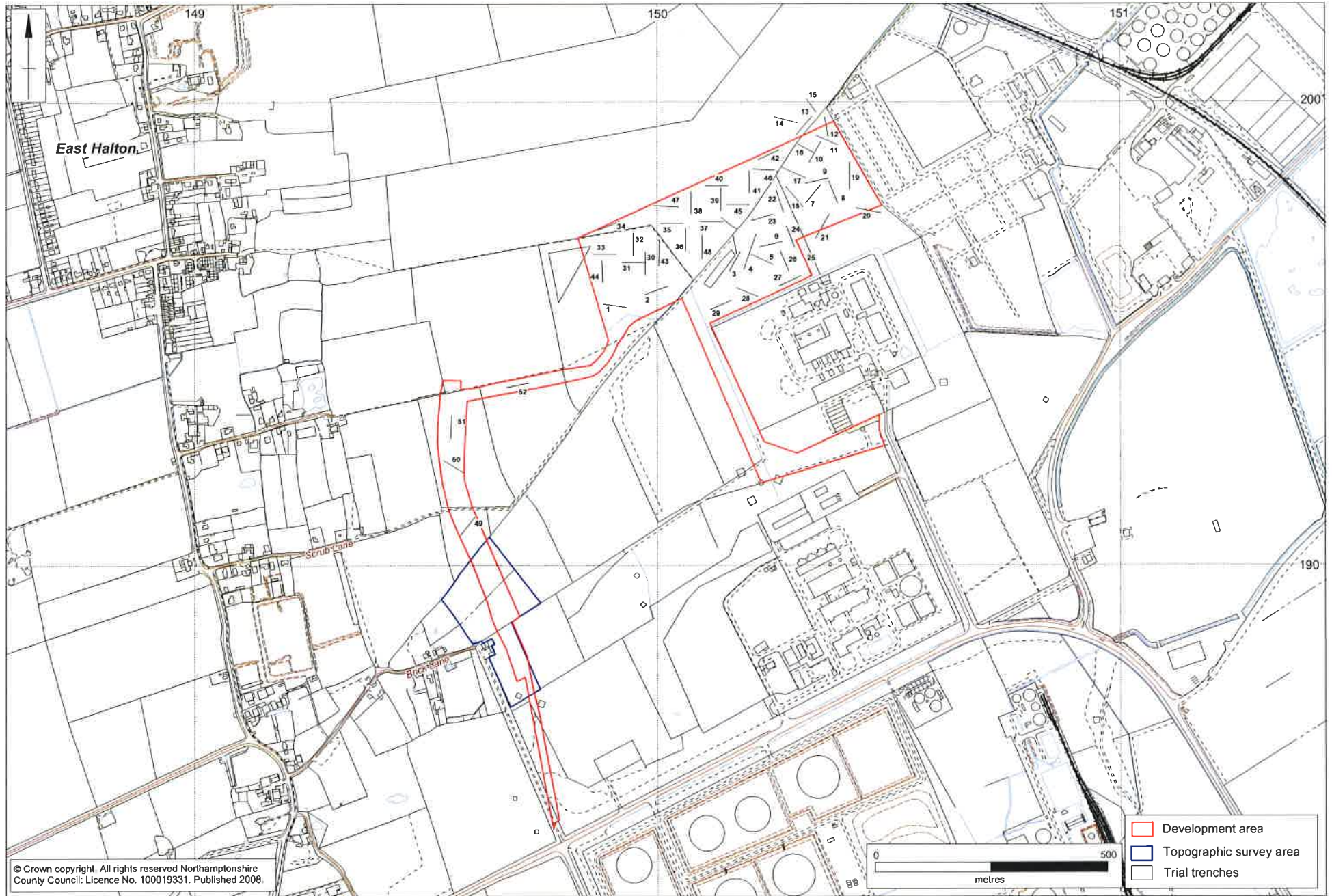
Trench and topographic survey locations Fig 2
