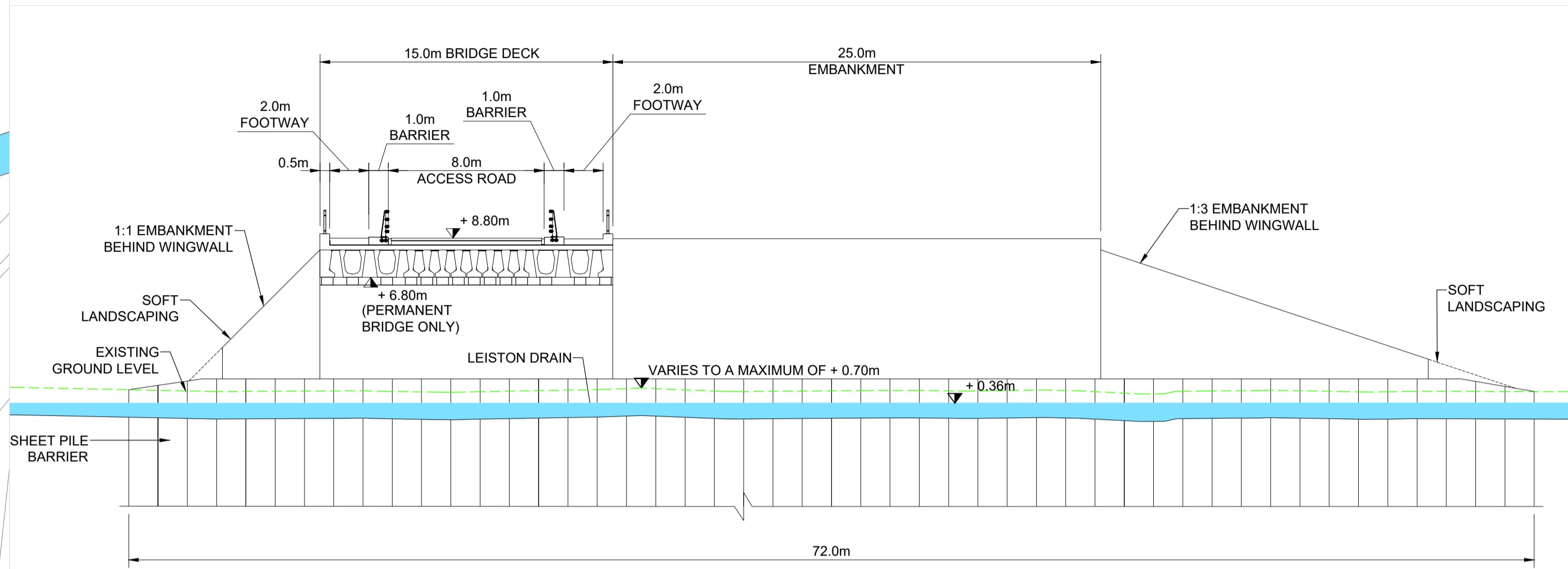
SECTION B - B SCALE 1:200
