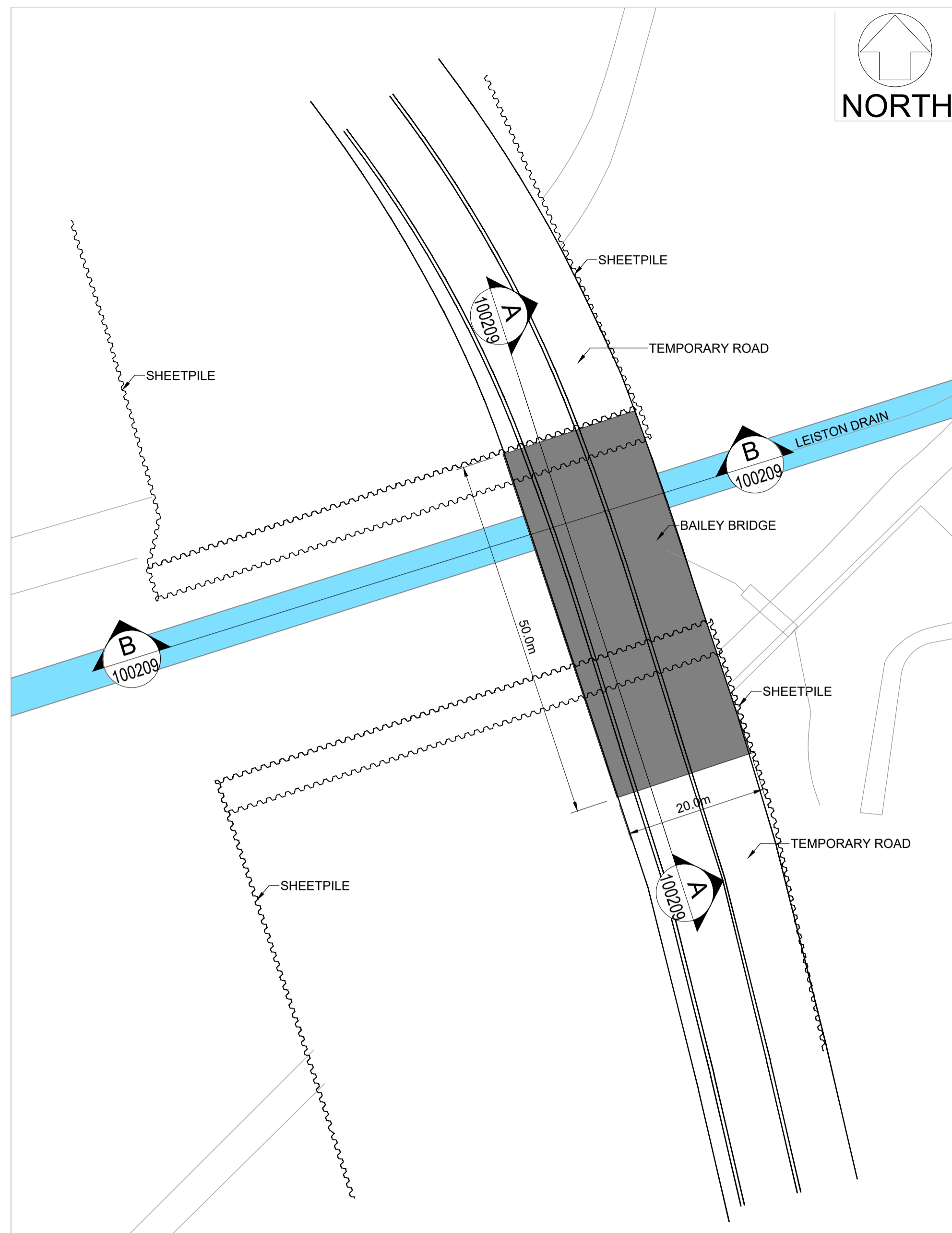
PLAN SCALE:1:500
