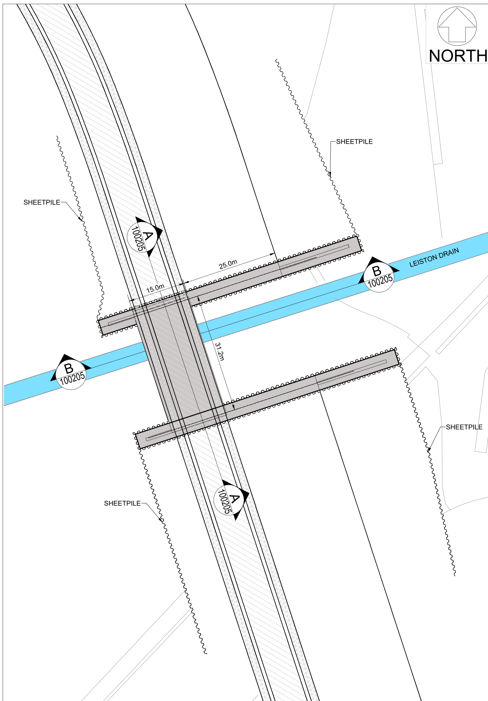
PLAN SCALE:1:500
