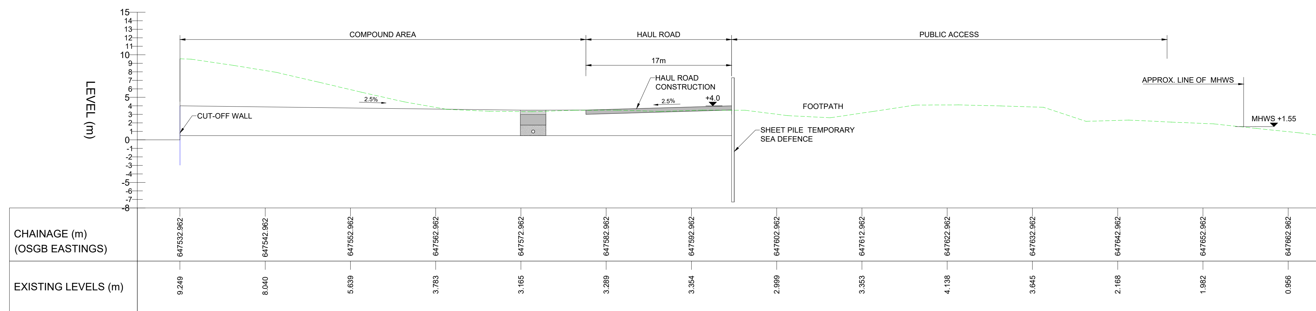
SECTION @ D - D CONSTRUCTION SITE - DURING CONSTRUCTION OF MAIN DEVELOPMENT SITE SCALE 1:250
