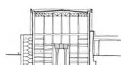
Section through Turbine Hall showing internal operations
