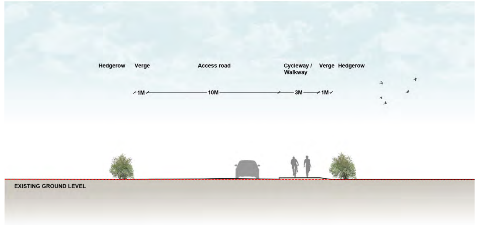
Section O-O'
