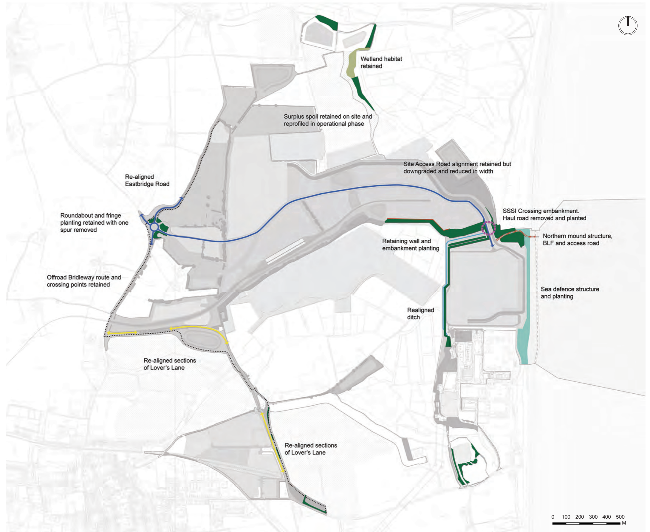
Figure 8.6: Inheritance from Construction Masterplan (Indicative) reprofiled in operational phase where possible
