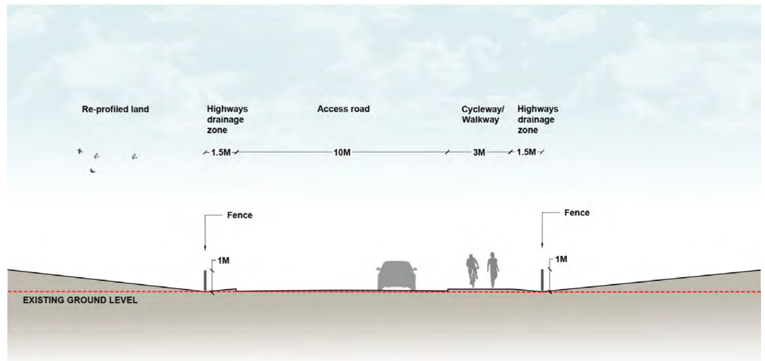
Section P-P'
