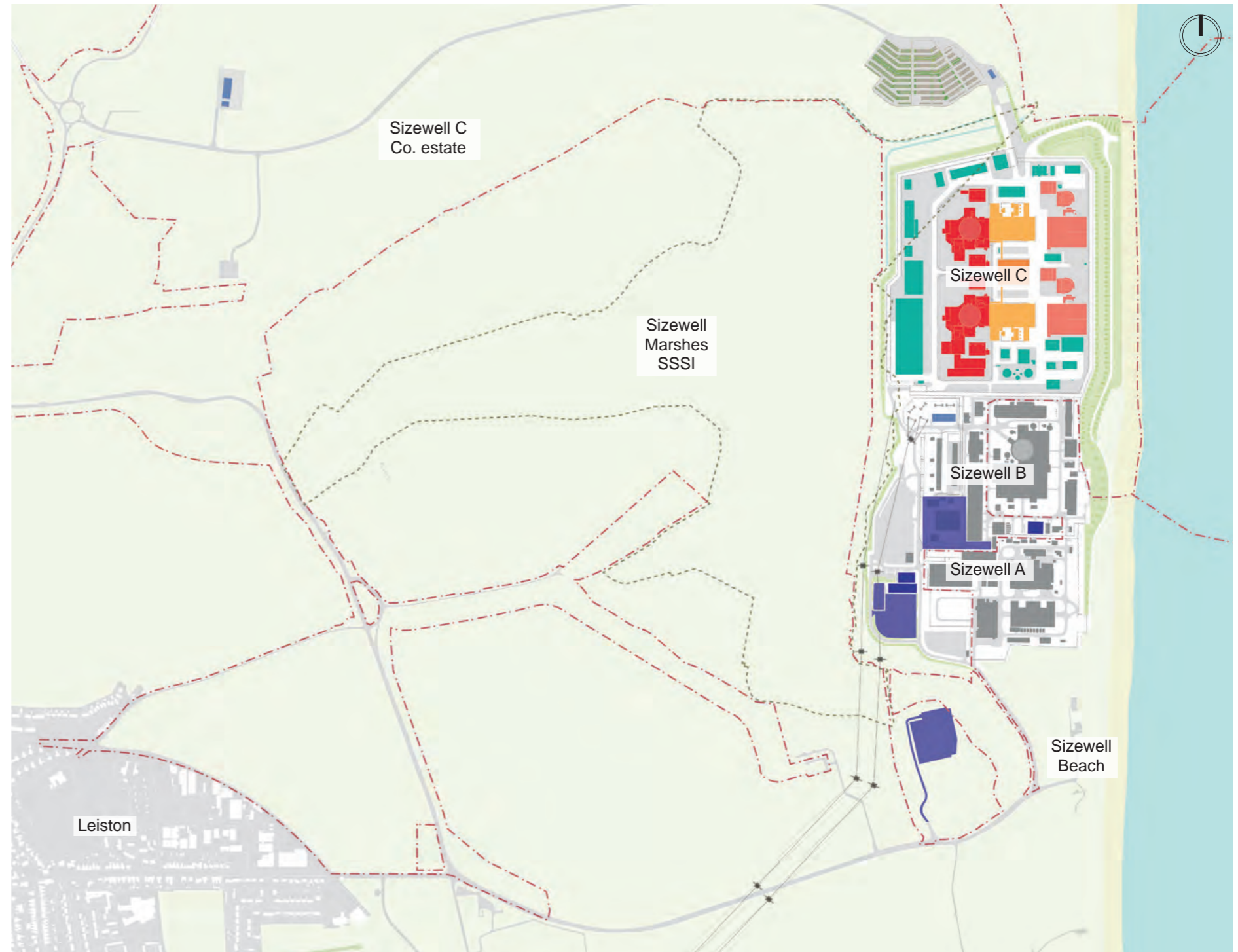
Figure 7.3: Proposed Sizewell C buildings and structures within the SZC Co. operational masterplan
