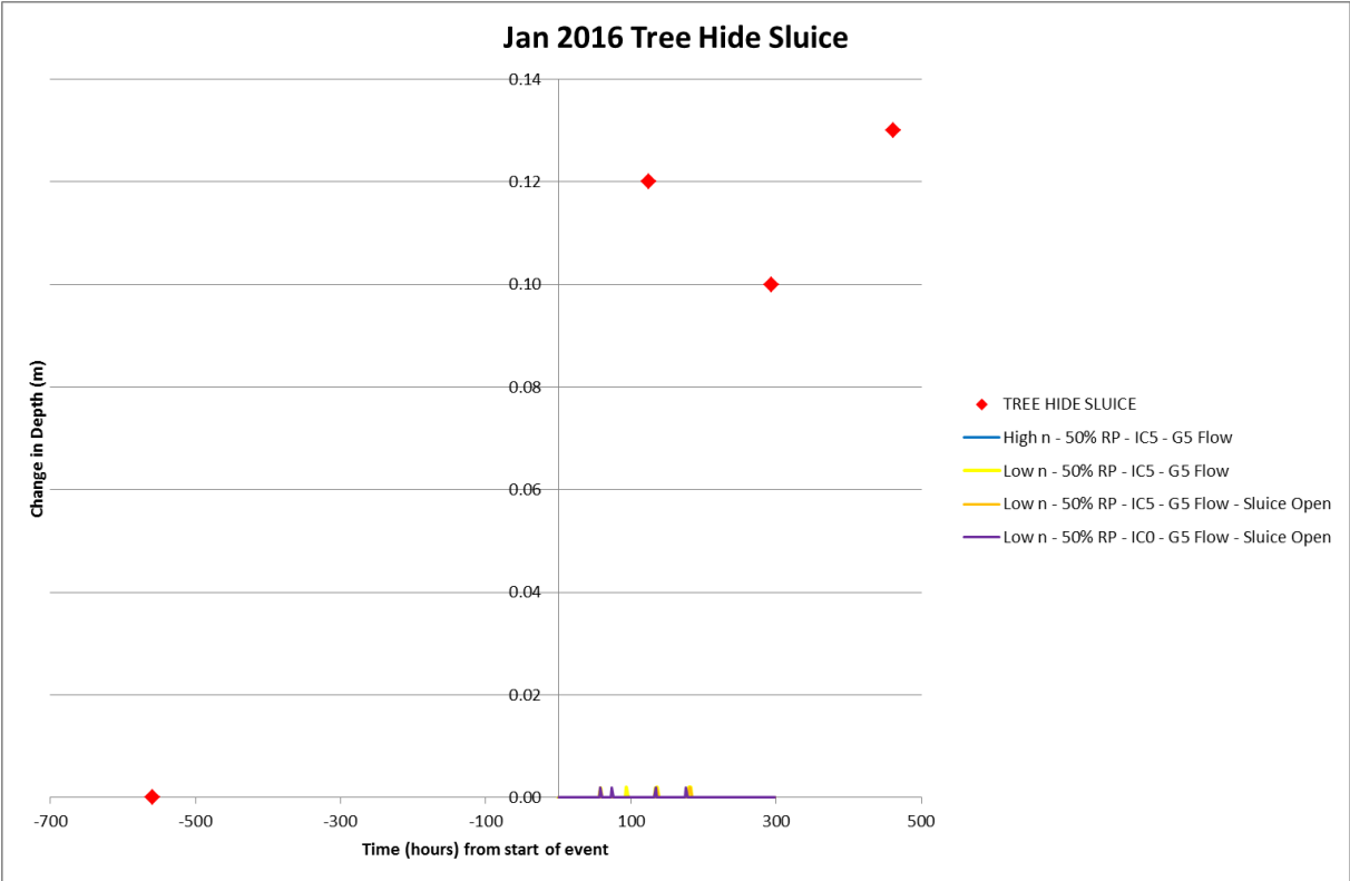
Figure 1 - January 2016 Tree Hide Sluice Changes in Modelled and Observed Water Depth
