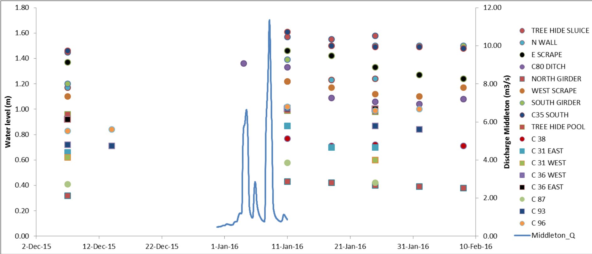
Figure showing the data availability for the Minsmere system (for each gauging station) during the 2016 event. It shows that no data is available during the event for the entire Minsmere system and that the only data that is available is weekly data. As the events duration is little over a week this is of little help.
